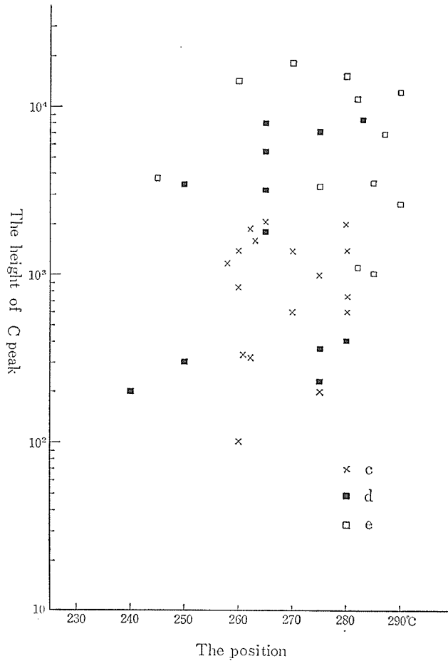
Fig. 4. Variation of the height and the position of C peak in quartz from various rocks after 10^7 r irradiation. c: quartz from granite, d: quartz from pegmatite, e: quartz from druse in pegmatite.
