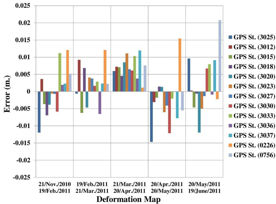
Fig.9. Deformation maps errors at GPS stations
