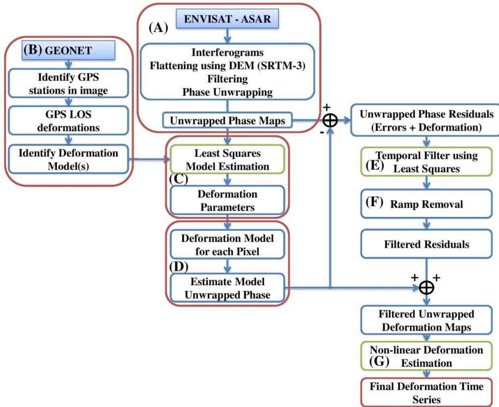
Fig.3. Methodology block diagram
