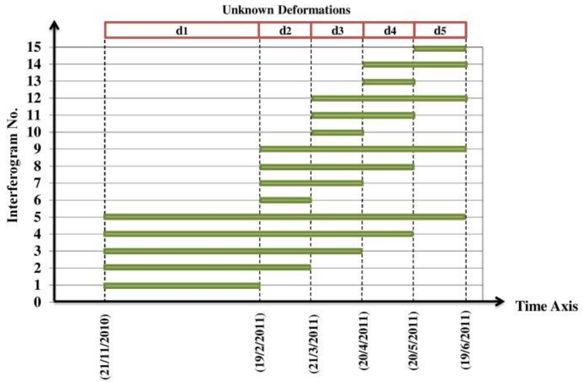
Fig.5. Interferograms stack structure, each bar represents an interferogram with the right end at the master image acquisition date and the left end at the slave image acquisition date.
