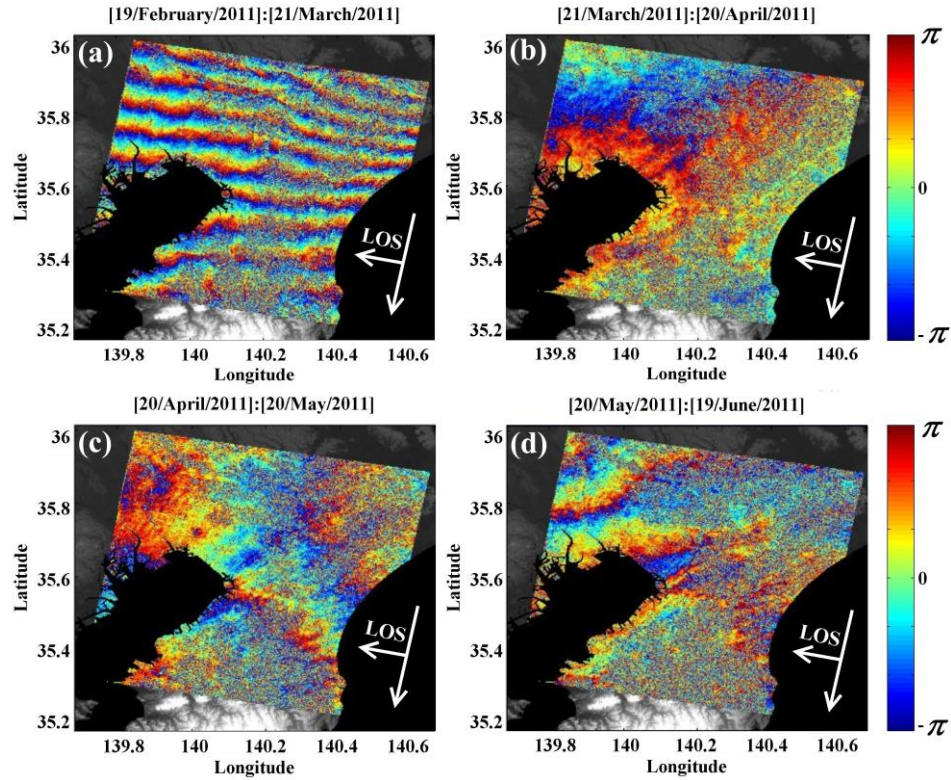
Fig.2. Interferograms using ENVISAT-ASAR C-band images, each fringe cycle equivalent to a displacement of 2.8 cm. (a) coseismic interferogram [19/Feb/2011 : 21/March/2011], and postseismic interferograms (b) [21/March/2011 : 20/April/2011], (c) [20/April/2011 : 20/May/2011], (d) [20/May/2011 : 19/June/2011], background is a DEM map.
