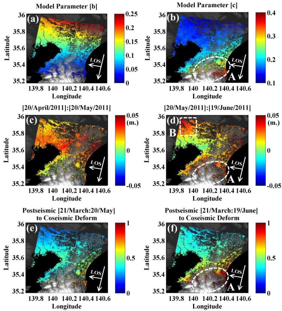
Fig. 11. (a) Multiplication model paramter [b], (b) power model paramter [c], (c) postseismic deformation map [20/April/2011 : 20/May/2011],(d) postseismic deformation map [20/May/2011 : 19/June/2011], (e) ratio between the postseismic deformation up to May 20 th , 2011 and the coseismic deformation, (f) ratio between the postseismic deformation up to June 19 th , 2011 and the coseismic deformation, background is a DEM map.
