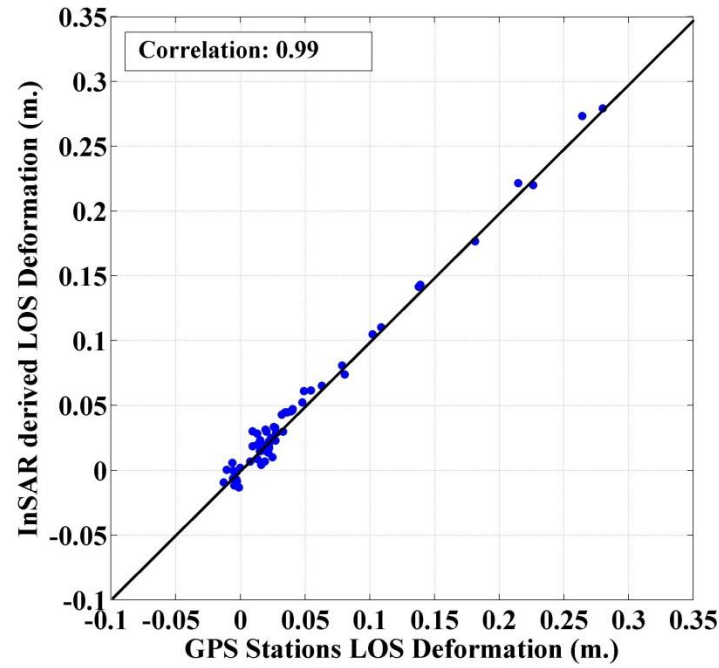
Fig.10. InSAR LOS deformations obtained by GPS against deformations obtained by InSAR
