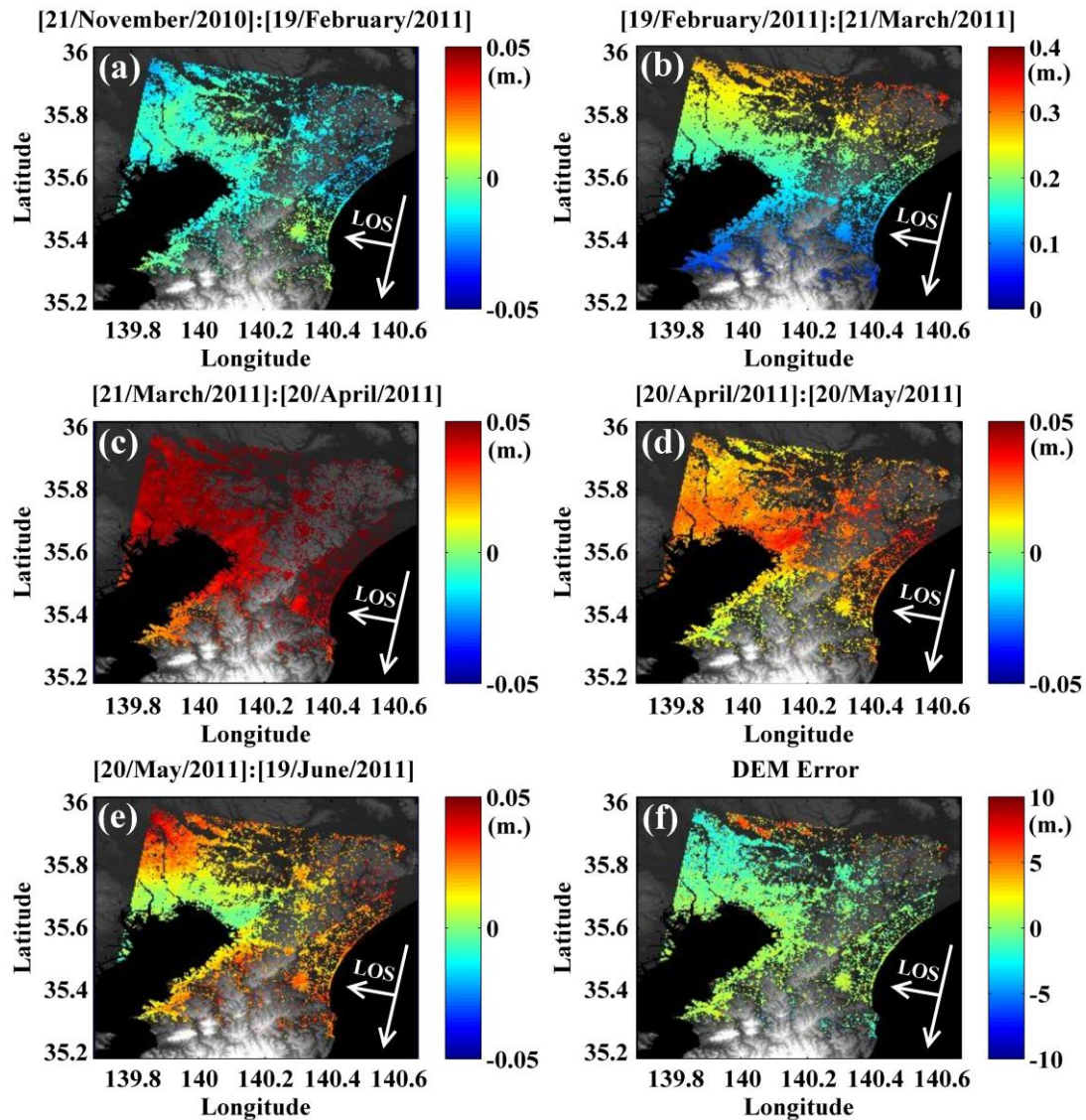
Fig.7. [a : e] Final deformation maps, [f] DEM error, background is a DEM map.
