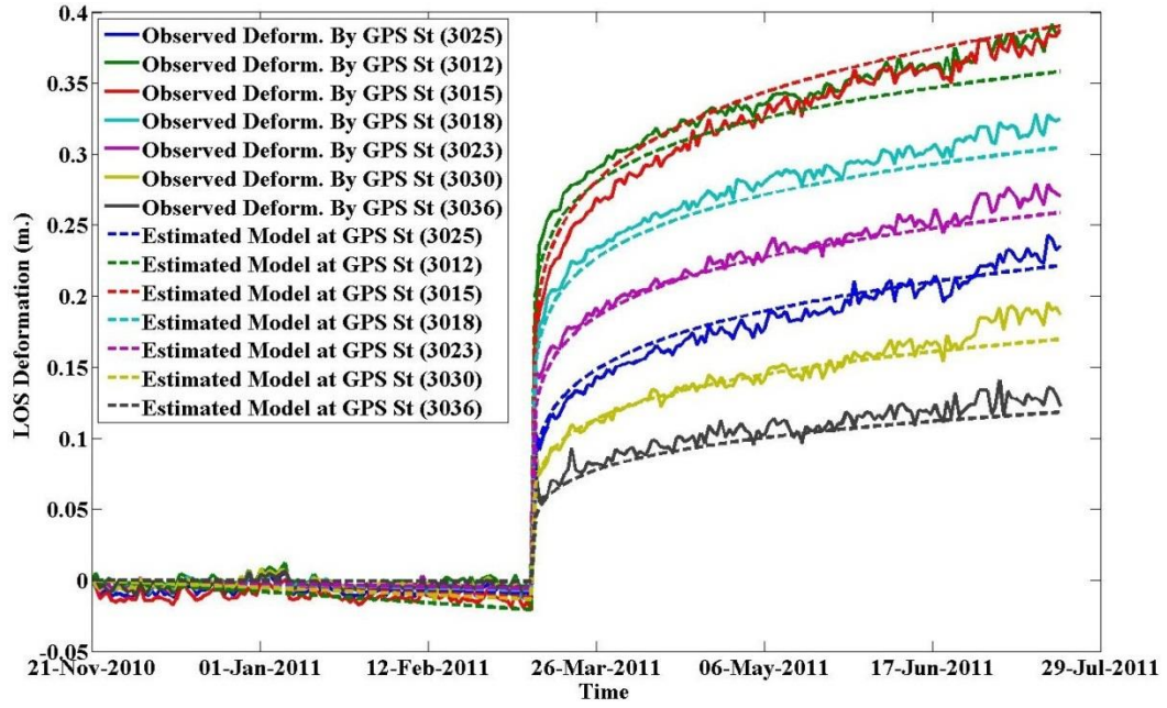
Fig.6. Observed LOS deformations and estimated deformation trends at GPS stations (descending direction).
