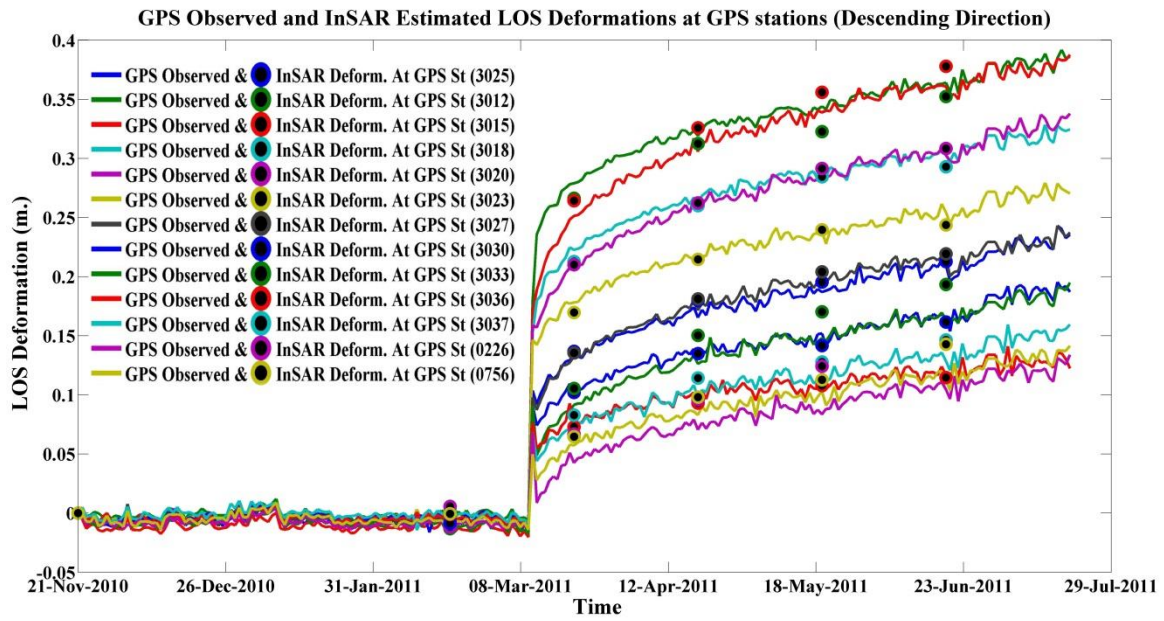
Fig.8. GPS observed deformations (solid lines) against InSAR estimated deformations (dots) in LOS descending direction at 13 GPS stations.
