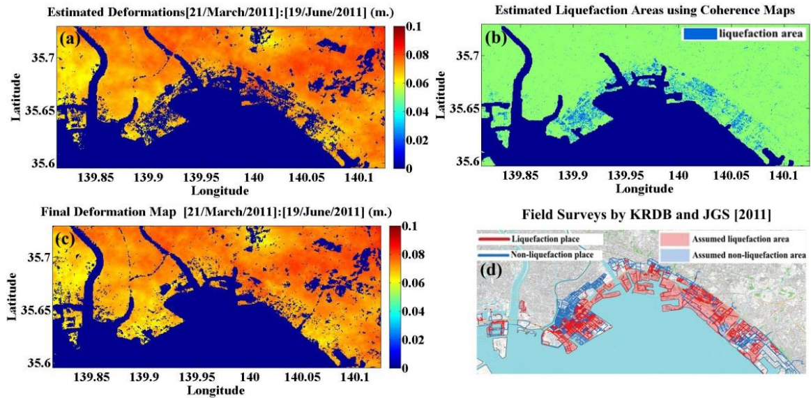
Fig. 13. (a) Postseismic deformation maps using the proposed method, (b) Liquefaction areas using the coherence difference method, (c) Final postseismic deformation maps, (d) Observed liquefaction through field surveys conducted by KRDB and JGS (2011).
