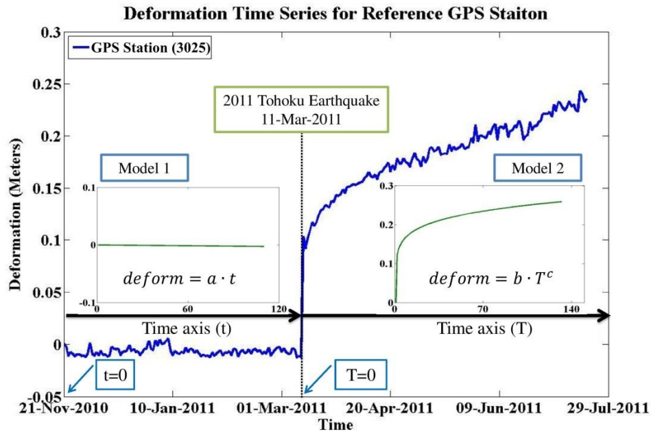
Fig.4. Observed LOS deformation using GPS station no. 3025 and the proposed deformation trends.
