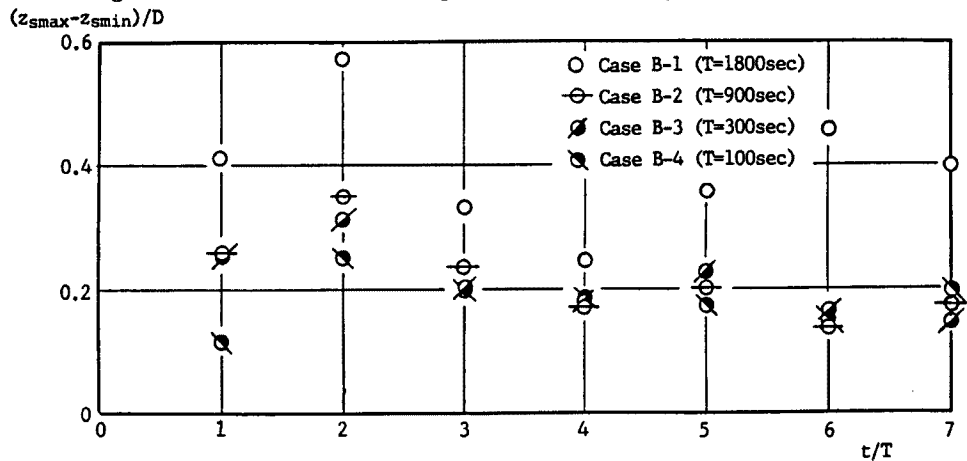
Fig. 4. Amplitude of the variation of scour depth.
