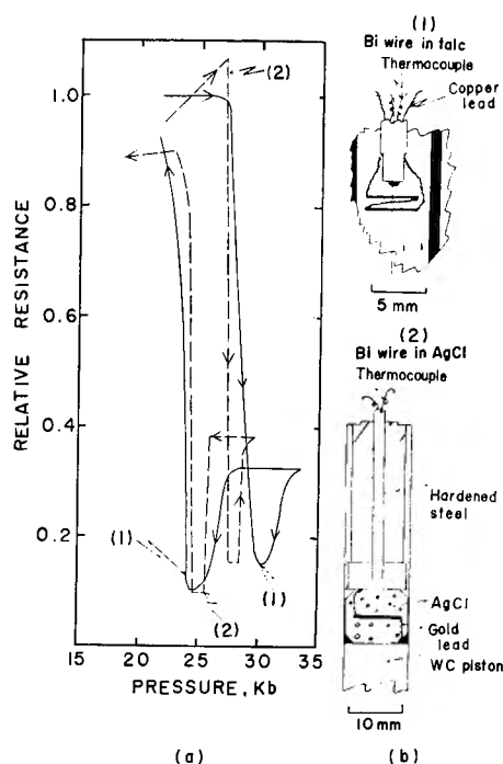
Fig. 2. (a) Typical cycles through the transition of bismuth wire embedded in talc at 14°C (1), and in silver chloride at 21°C (2). (b) The respective sample arrangements.
