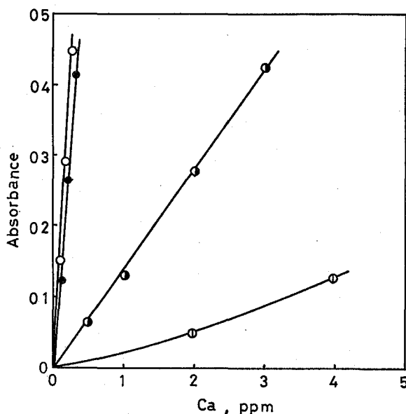
Fig. 13. Calibration curves for calcium. Height: 15 mm, radius: 2 mm, ○: atom line (4226.7 Å); Ca, ●: atom line (4226.7 Å); Ca + Na 300 ppm, ●: ion line (3933.7 Å); Ca + Na 120 ppm, ○: ion line (3968.5 Å); Ca + Na 120 ppm.
