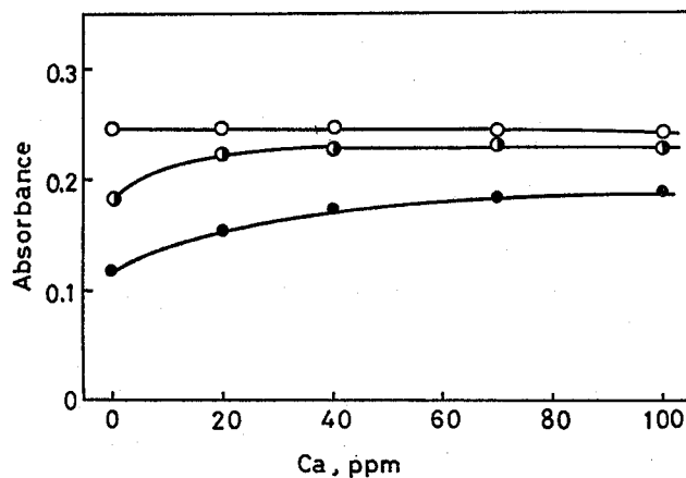
Fig. 7. Effect of varying concentrations of calcium chloride on absorbance of magnesium in the presence and absence of sodium.
