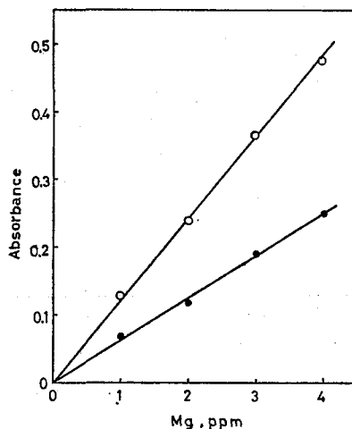
Fig. 5. Calibration curves for magnesium. ●; Mg, ○; Mg + Na 50 ppm.
