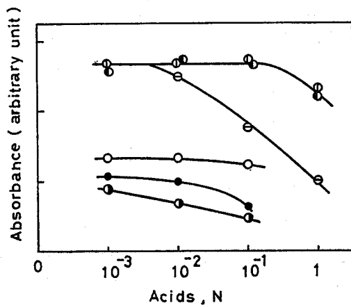
Fig. 6. Effect of increasing amounts of mineral acids on the absorbance of magnesium in the presence and absence of sodium chloride.
