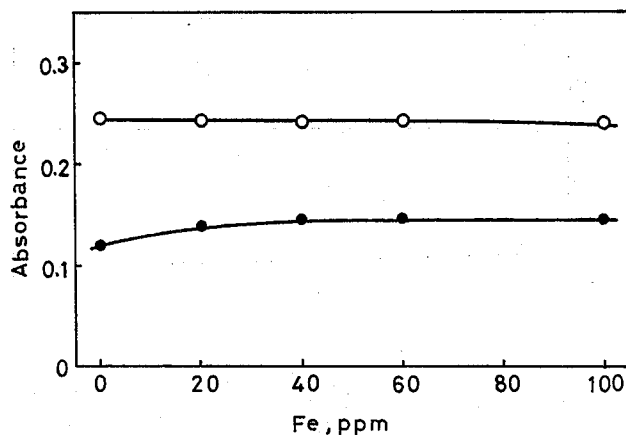
Fig. 8. Effect of varying concentrations of ferric chloride on absorbance of magnesium in the presence and absence of sodium.
