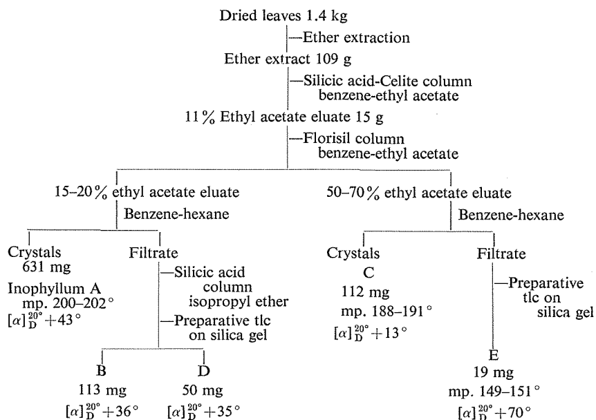
Fig. 1. Isolation procedure of the piscicidal constituents.
