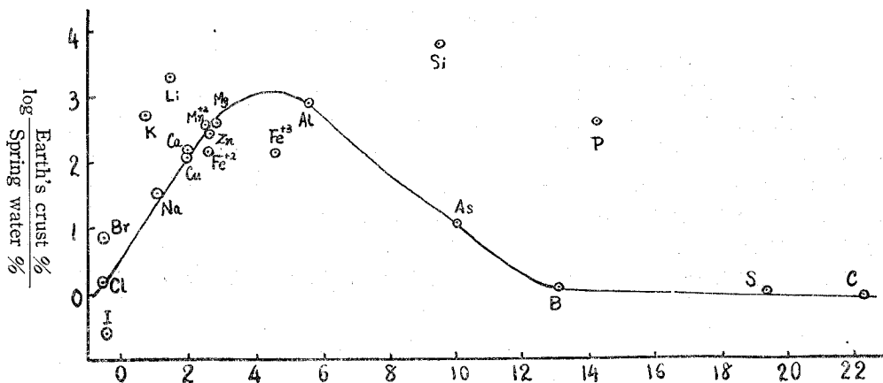
Fig. 3. Ionic Potential
