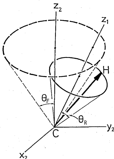
Fig. 1. A schematic diagram of the multiple-correlation-time model corresponding to the case of p=3 .
