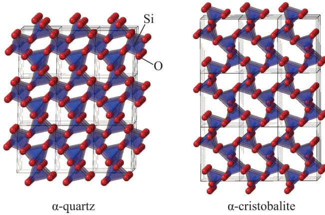
FIG. 1. Crystal structures of \alpha quartz (left) and \alpha cristobalite (right). The space-group types are P3_121 and P4_12_12 , respectively.
