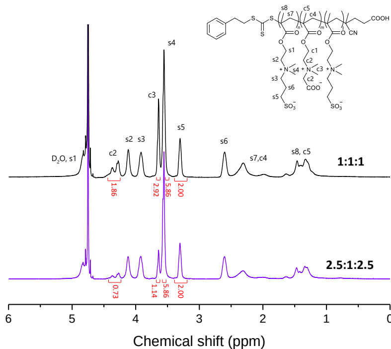
Figure 6.11. ^1\text{H} NMR spectra of two triblocks in \text{D}_2\text{O} at 60^\circ\text{C} . \text{SPE}_{198}\text{-GLBT}_{198}\text{-SPE}_{212} (target ratio = 1:1:1, black line) and \text{SPE}_{248}\text{-GLBT}_{99}\text{-SPE}_{277} (target ratio = 2.5:1:2.5, blue line)
