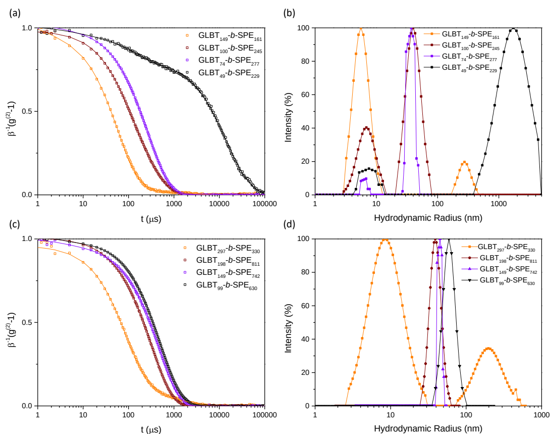
Figure 6.6. ACFs ((a) and (c)) and CONTIN analysis results ((b) and (d)) of PGLBT- b -PSPE aqueous solutions having different block ratios and total chain length. (a) and (b): DP_{\text{total}} = \sim 300 , (c) and (d): DP_{\text{total}} = \sim 600 . The ACFs and size distributions are obtained at 90°, 12 °C.
