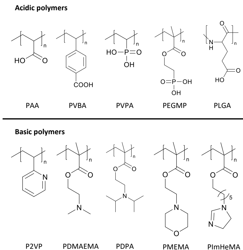
Figure 1.8. Examples of pH-responsive polymers
