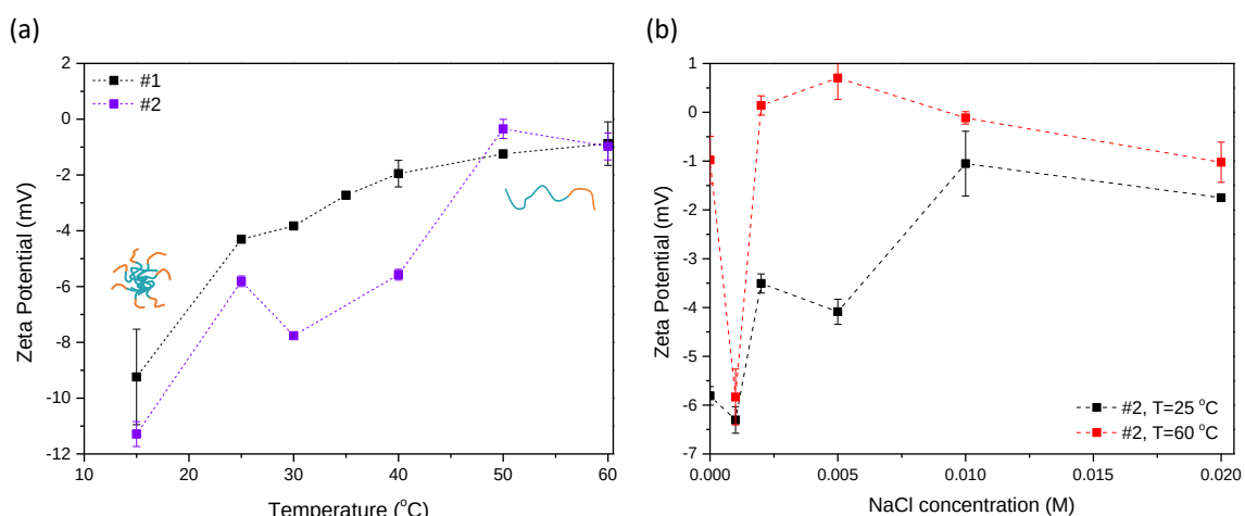
Figure 3.7. (a) Zeta potential variations of PGLBT- b -PSPEs against temperature (black: #1, violet: #2) (b) Zeta potential variations of #2 against [NaCl] at 25\text{ }^{\circ}\text{C} (micelle state) and 60\text{ }^{\circ}\text{C} (unimer state)
