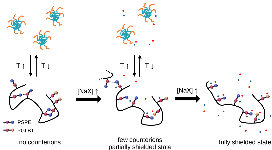
Scheme 3.2. A Proposed model of PGLBT- b -PSPE incorporated with salt ions in water. (dashed line: possible zwitterionic attraction, red dot: cations ( Na^+ ), blue dot: halides ( X^- : F^- , Cl^- , Br^- , and I^- ))
