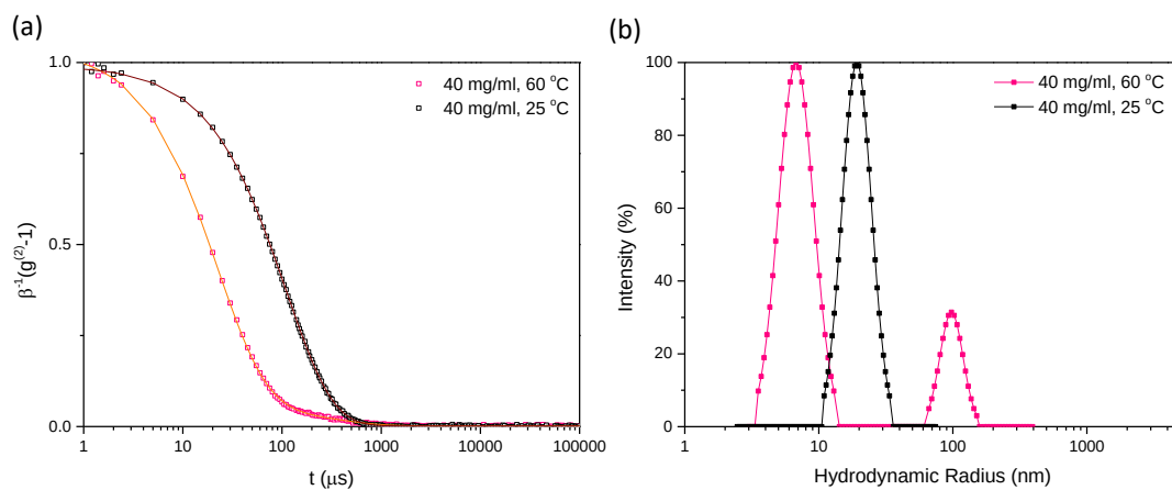
Figure 6.12. (a) ACFs and (b) the CONTIN analysis result of \text{GLBT}_{49}\text{-b-SPE}_{229} solution (conc. = 40 mg/mL) measured at 25 and 60^\circ\text{C} , respectively.
