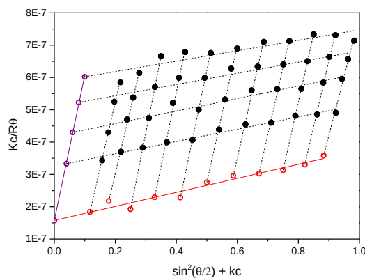
Figure 3.12. Zimm plot obtained by SLS of #2 in 20 mM NaCl (aq) at 12 °C. R_{g,c=0} = 77 nm, A_2 = 2.25 \times 10^{-5} cm 3 mol/g 2 ( dn/dc of #2 = 0.1445 mL/g). The R_g of respective concentrations are as follows: 10 mg/mL: 31.9 nm, 8 mg/mL: 35.9 nm, 6 mg/mL: 40.4 nm, 4 mg/mL: 49.5 nm
