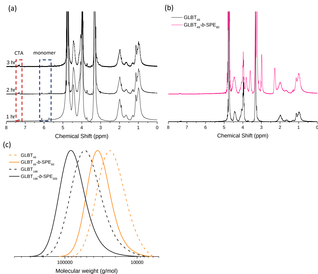
Figure 5.1. (a) ^1H NMR spectra of GLBT_{49} taken at 1 h intervals. (b) ^1H NMR spectra of GLBT_{49} (black) and GLBT_{49} - b - SPE_{60} (red) obtained from aliquots withdrawn after 3 h (c) MWDs of GLBT_{49} and GLBT_{49} - b - SPE_{60} , and GLBT_{198} and GLBT_{198} - b - SPE_{305} by SEC analysis
