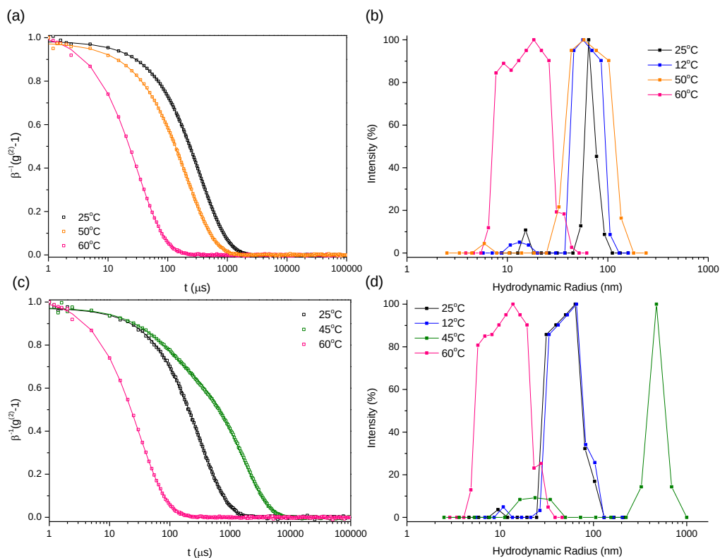
Figure 2.12. Autocorrelation functions (ACF) of PGLBT- b -PSPEs and hydrodynamic radius distribution of PGLBT- b -PSPEs obtained by CONTIN analysis at 90°. (a) PGLBT 182 - b -PSPE 204 , ACF (b) PGLBT 182 - b -PSPE 204 , CONTIN analysis (c) PGLBT 131 - b -PSPE 193 , ACF (d) PGLBT 131 - b -PSPE 193 , CONTIN analysis
