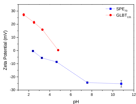
Figure 4.14. Zeta potential of two homo-polybetaines: SPE 70 and GLBT 131 under varying pH
