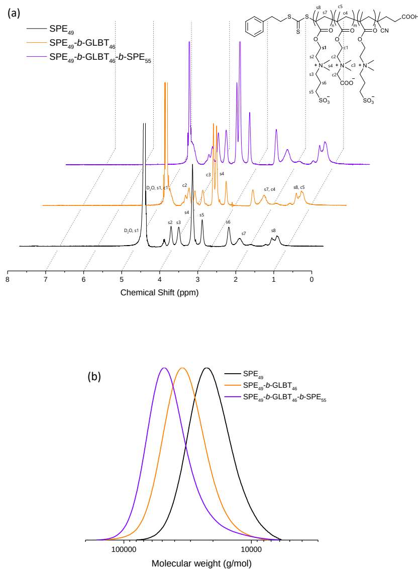
Figure 5.4. (a) ^1\text{H} NMR spectra (obtained at 60 °C) of \text{SPE}_{49}\text{-}b\text{-GLBT}_{46}\text{-}b\text{-SPE}_{55} on each synthesis step (b) MWDs by SEC analysis of \text{SPE}_{49}\text{-}b\text{-GLBT}_{46}\text{-}b\text{-SPE}_{55}
