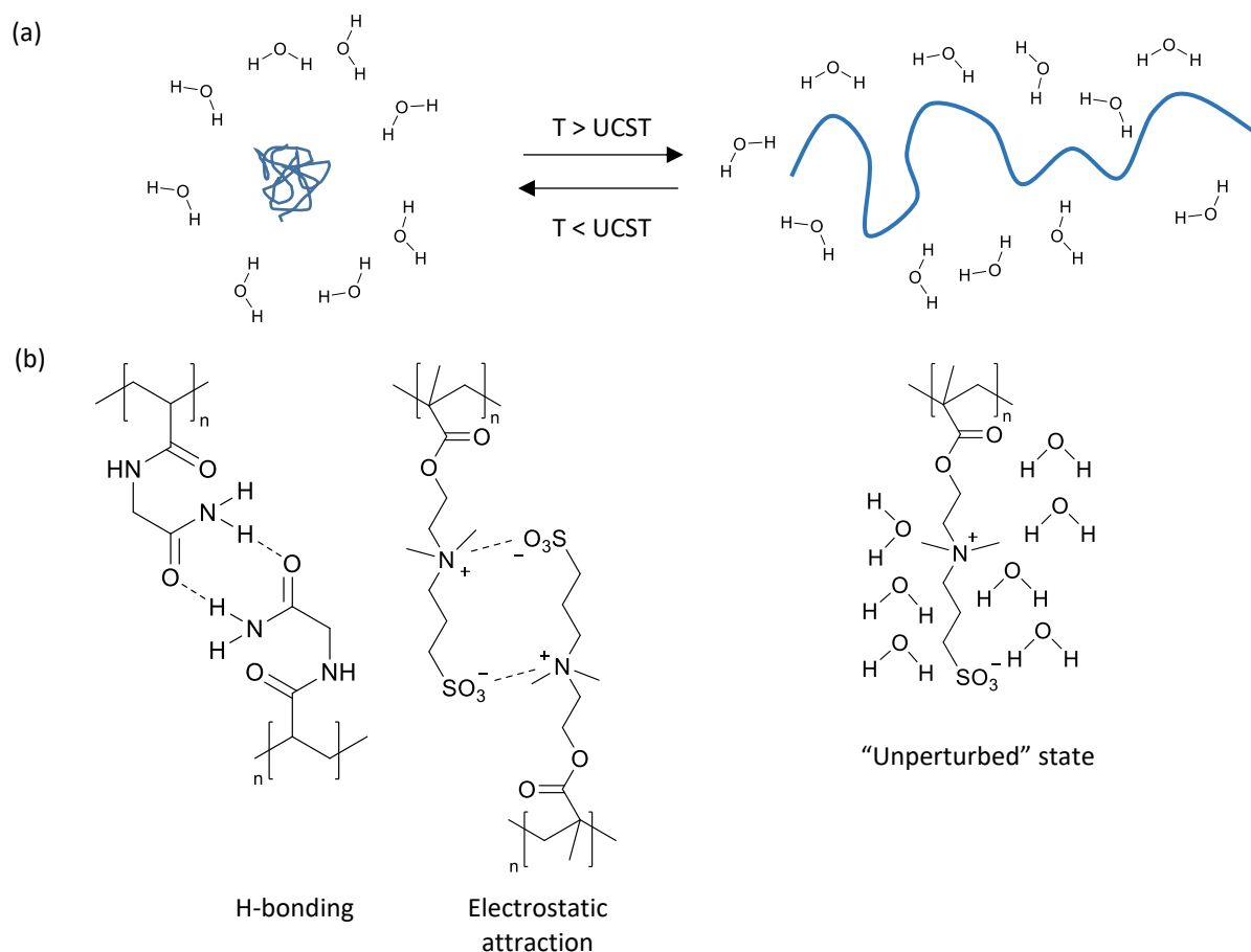
Figure 1.5. (a) Schematic view of phase behaviour of UCST polymers (b) Chemical structures representations of UCST polymers in a phase separated and dissolved state (Left: the cohesive force is H-bonding for PNAGA and electrostatic attraction for PSPE Right: the original ordering of water molecules are not disturbed by dissolution of polysulfobetaines)
