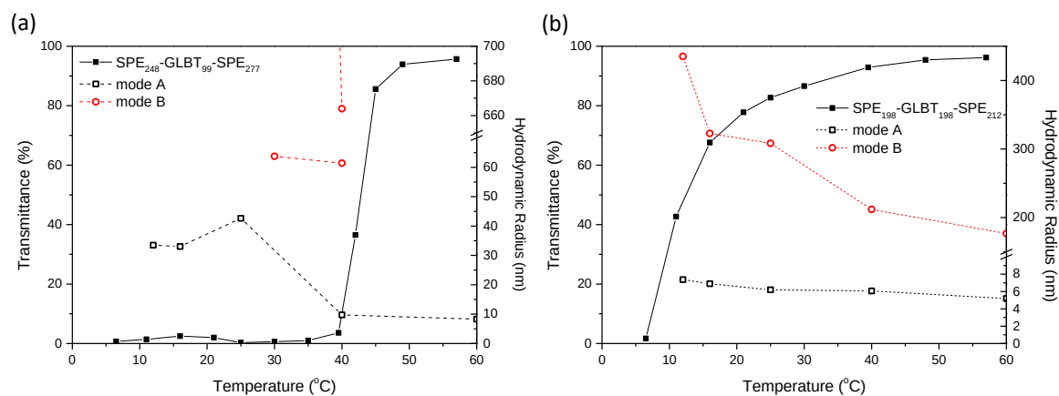
Figure 6.8. Variations of transmittance (■) and R_h (open symbols) against temperature of triblock betaine copolymers (a) \text{SPE}_{248}\text{-GLBT}_{99}\text{-SPE}_{277} (b) \text{SPE}_{198}\text{-GLBT}_{198}\text{-SPE}_{212}
