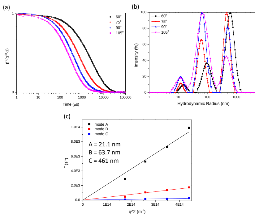
Figure 3.11. (a) DLS autocorrelation functions of #2 in 20 mM NaCl (aq) at four different angles of 60°, 75°, 90°, and 105° at T = 25 °C (b) Size distribution of hydrodynamic radii calculated by CONTIN (c) The decay rate \Gamma versus q^2 of three diffusive modes obtained at multiple scattering angles
