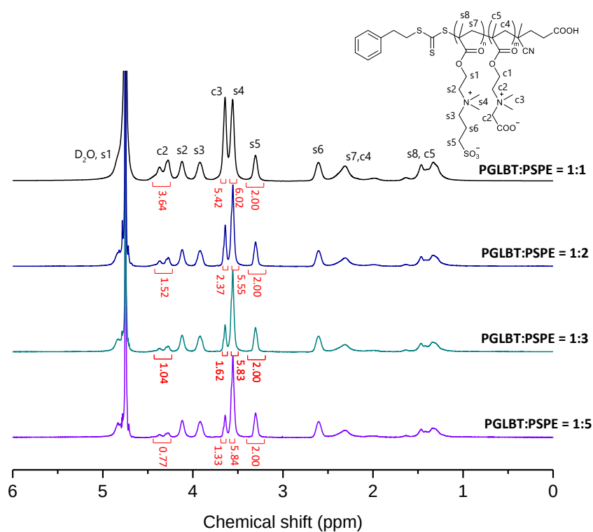
Figure 6.1. ^1\text{H} NMR spectra of 4 PGLBT- b -PSPEs having several ratios acquired in \text{D}_2\text{O} at 60^\circ\text{C} ( \text{DP}_{\text{total}} \approx 300 )
