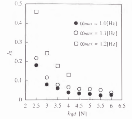
(b) J_g for grasping
