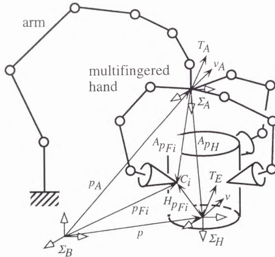
Fig. 6.1. Arm-hand mechanism.
