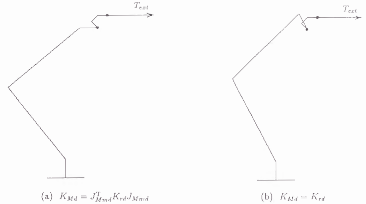
Fig. 5.5. Final posture of macro-micro manipulator.
