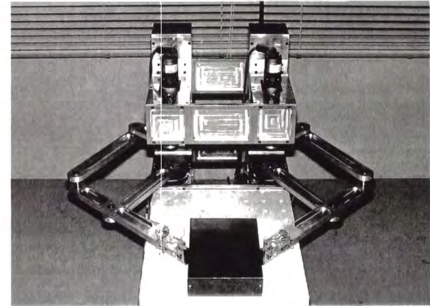
Fig. 4.5. Experimental setup.
