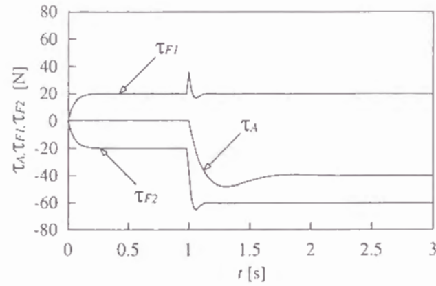
(e) Joint force
