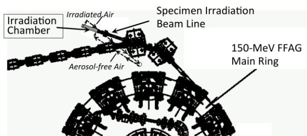
Fig.1 Irradiation Chamber
