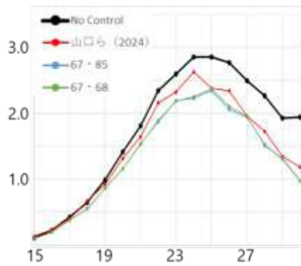
Fig. 29 Time series of the maximum rainwater mixing ratio [g/kg] at 67・68 and 67・85 in Sensitivity Experiment B-3. The horizontal axis represents the elapsed time [minutes], and the vertical axis shows the maximum rainwater mixing ratio [g/kg] at that time.
