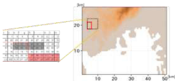
Fig. 12 The position with the greatest suppression effect obtained in Sensitivity Experiment A-1 (gray area), the position used by Yamaguchi et al. (2024) (light red area), and the location of the potential temperature bubble (red box). Details about the English labels and specific positions in the figure will be explained in Sensitivity Experiment A-2.
