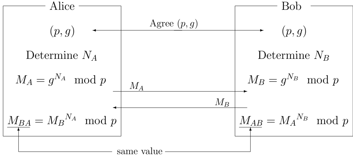
Figure 2.2: Diffie-Hellman key-exchange
