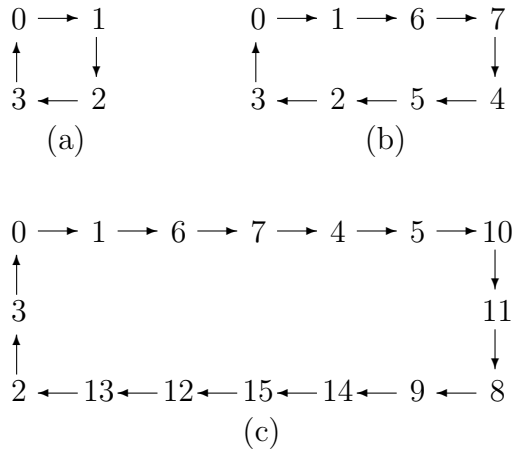
Figure 4.1: Orbits passed by F(X) . (a) Orbit on \mathbb{Z}/2^2\mathbb{Z} . (b) Orbit on \mathbb{Z}/2^3\mathbb{Z} . (c) Orbit on \mathbb{Z}/2^4\mathbb{Z} .
