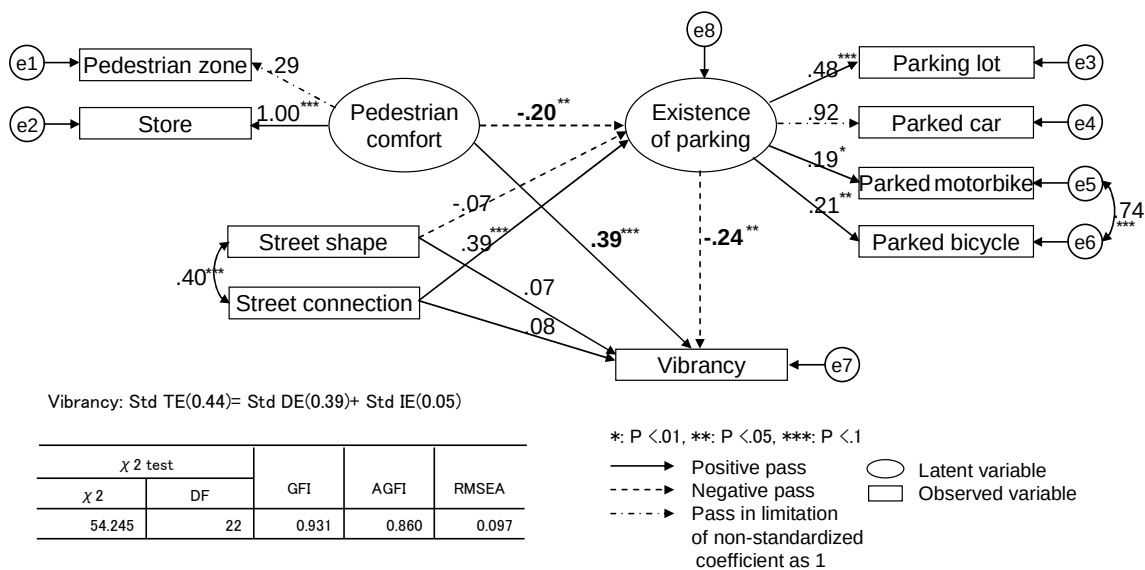
Figure 87 Structural Equation Model in Beijing
