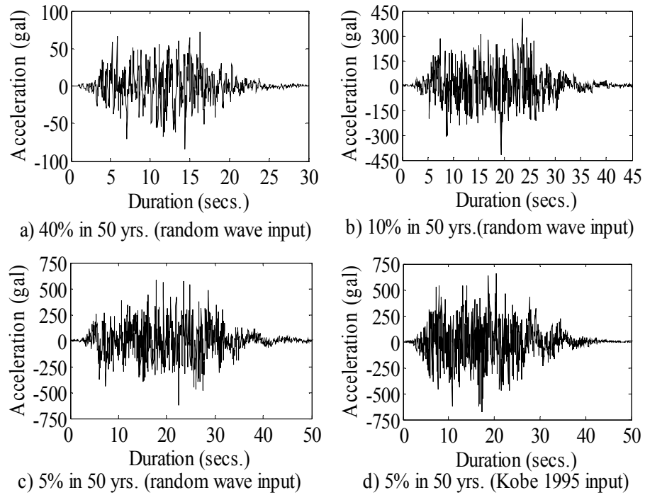
Fig. 3.4 Simulated acceleration histories for various return periods
