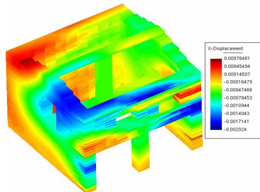
Fig. 6.22 Deformations in model 4 under 98 yrs RT earthquake
