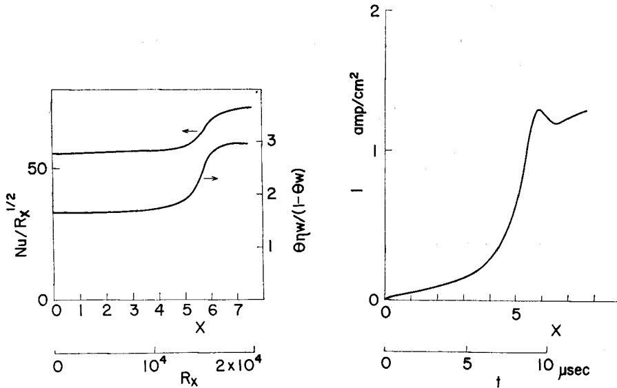
Fig. 9. Variation of Nusselt number in the region behind a shock wave.
