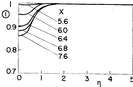
Fig. 7. Electron temperature profiles in the boundary layer.
