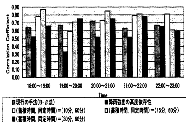
Fig. 11 Correlation coefficient above the points where the surface rainfall is observed.
