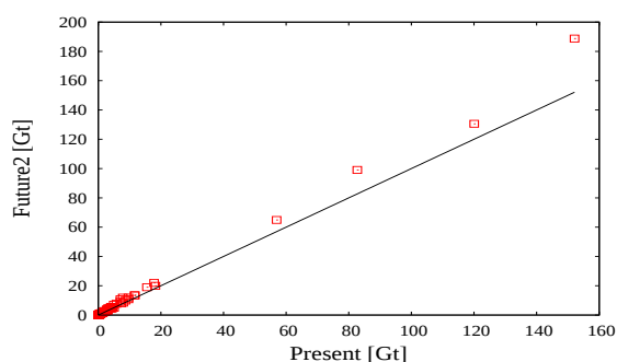
(a) 0-160 [Gt]
