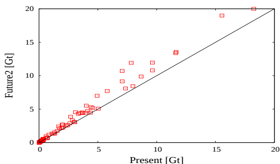
(b) 0-20 [Gt]
