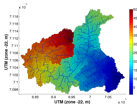
Fig. 10 Time classes spatially distributed using mean velocity, Cubatão River watershed
