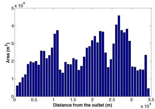
Fig. 5 Area-distance function for Pequeno River watershed
