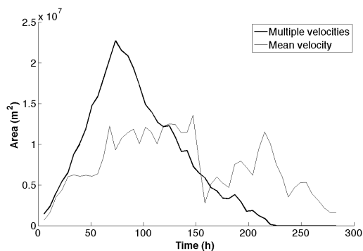
Fig. 7 Comparison between time-area functions, Cubatão River watershed
