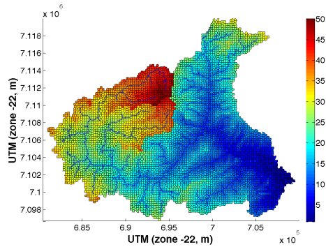
Fig. 13 Time classes spatially distributed using multi-velocities, Cubatão River watershed
