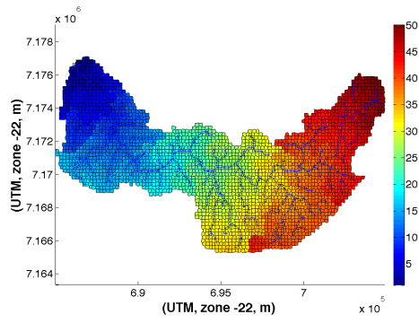
Fig. 11 Time classes spatially distributed using mean velocity, Pequeno River watershed
