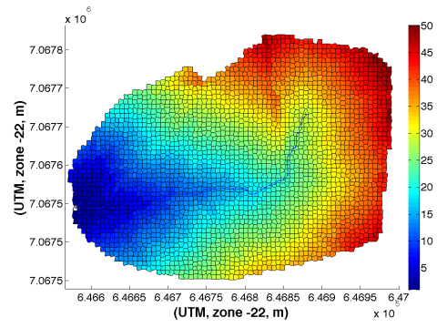
Fig. 15 Time classes spatially distributed using multi-velocities, Pinus I watershed
