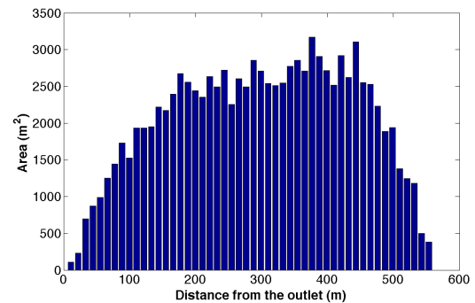
Fig. 6 Area-distance function for Pinus I watershed.
