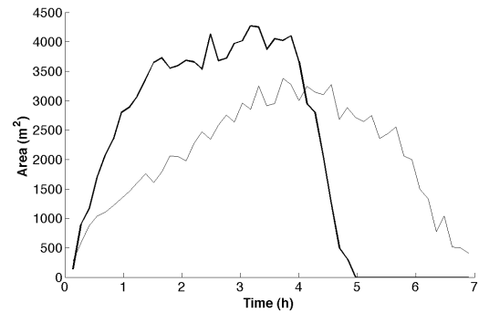
Fig. 9 Comparison between time-area functions, Pinus I watershed
