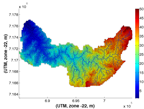
Fig. 14 Time classes spatially distributed using multi-velocities, Pequeno River watershed
