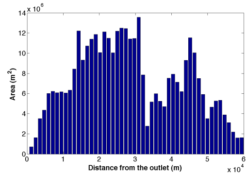
Fig. 4 Area-distance function for Cubatão River watershed
