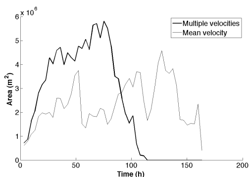
Fig. 8 Comparison between time-area functions, Pequeno River watershed
