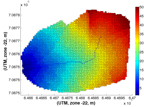
Fig. 12 Time classes spatially distributed using mean velocity, Pinus I watershed
