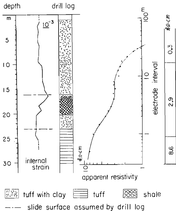
Fig. 3. Comparison of the depth of the slide surface measured by various methods (at Usagiguchi No. 5 drill hole of the Matsunoyama landslide).
