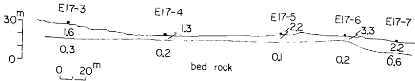
Fig. 2. Crustal structure at E-17 span in the Matsunoyama landslide (bed rock shown as under 0.3 \text{ k}\Omega\text{-cm} ).
