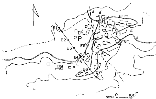
Fig. 4. Disposition of the instruments.
