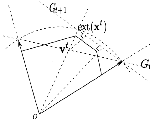
Figure 1: Similar triangles.
