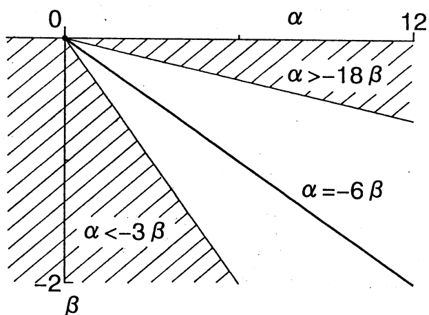
Fig. 3. Parameter region of \alpha and \beta , where analytical solitary wave solutions (3.17) can exist in the hatched region, while eq. (1.1) passes the Painlevé PDE test on the closed circle (•) and eq. (3.2) passes the Painlevé ODE test on the solid line.
