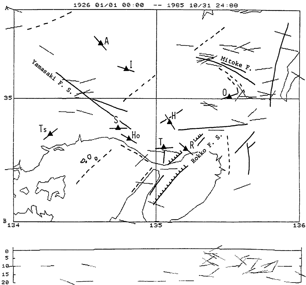
Fig. 1. Horizontal (upper) and vertical (lower) projections of P-axes of crustal earthquake ( H \leq 20 km) in Northern Kinki.
