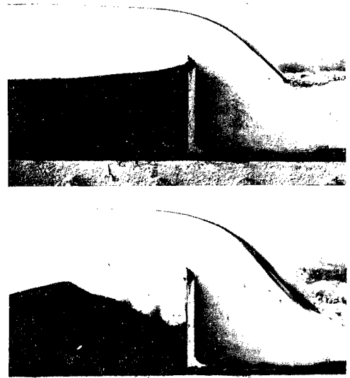
Photo. 1 View of bed and water profile near the weir
