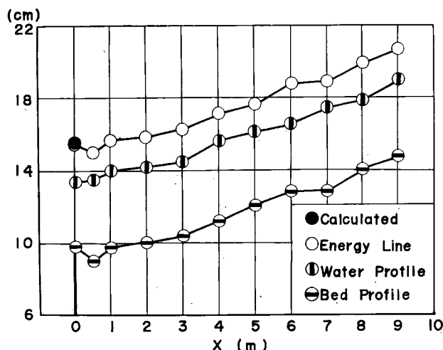
Fig. 5 Variation of elevation of bed, water level and energy head with distance
