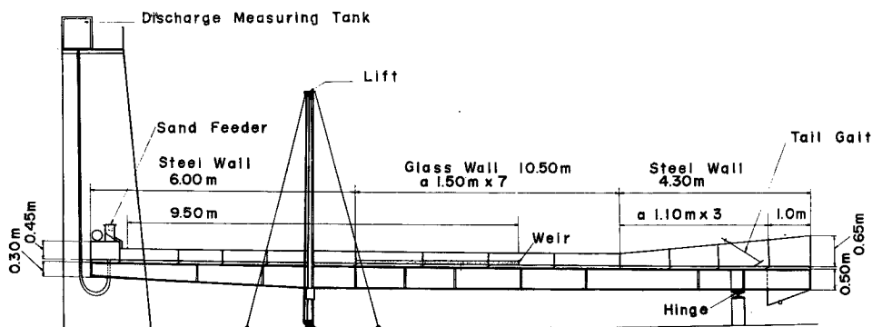
Fig. 2 Experimental flume
