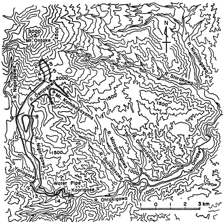
Fig. 1 The trace of soil block motion released by Ontake land slide
