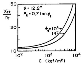
Fig. 13 Moving distance condition for a soil block to be a complete fluid motion
