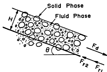
Fig. 8 Definition sketch of multi-phase flow
