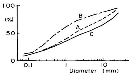
Fig. 3 Particle size distributions of sediment deposits transported by the catastrophic debris flow.
