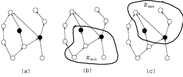
Fig. 2 Examples of R_{\min} and R_{\max} .
