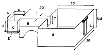
Fig. 3 Apparatus for heating gyre experiments (unit; cm).
