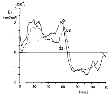
Fig. 12 Time variation of the buoyancy flux (Experiment).
