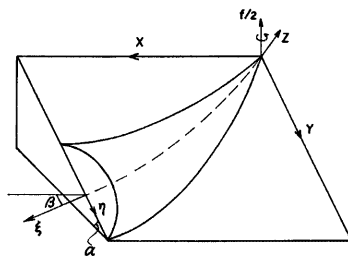
Fig. 23 The co-ordinate system for the Streamtube Model.
