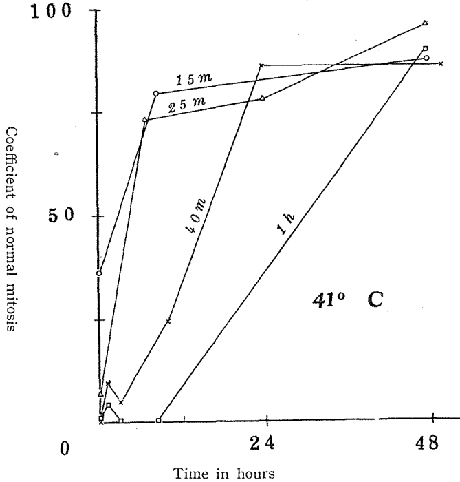
Text-fig. 9. Graphical presentation of the effect of heating at 41^{\circ}\text{C} on mitosis in the root tip cells of Vicia faba .
