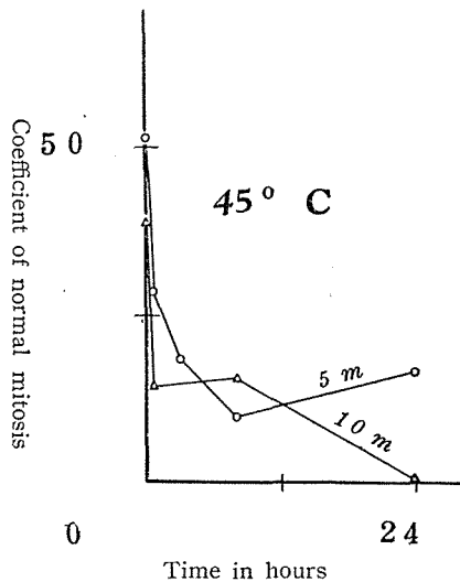
Text-fig. 11. Graphical presentation of the effect of heating at 45^{\circ}\text{C} on mitosis in the root tip cells of Vicia faba .
