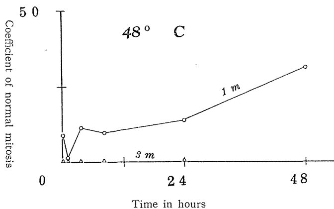
Text-fig. 12. Graphical presentation of the effect of heating at 48°C on mitosis in the root tip cells of Vicia faba .
