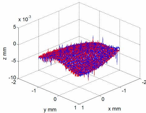
(c) Profile measurement error
