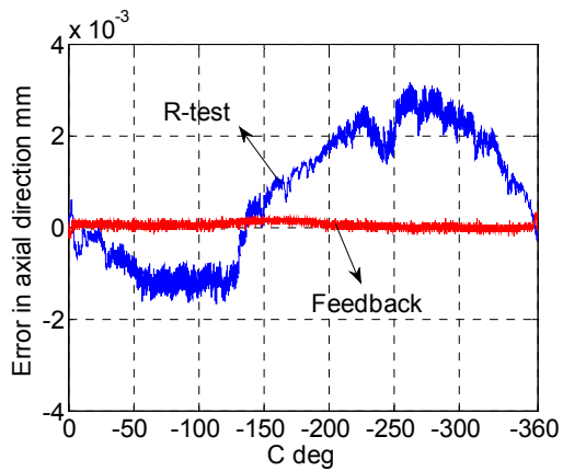
Contact-type R-test
