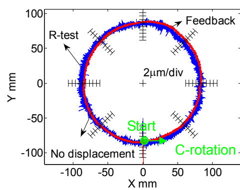
Non-contact R-test
