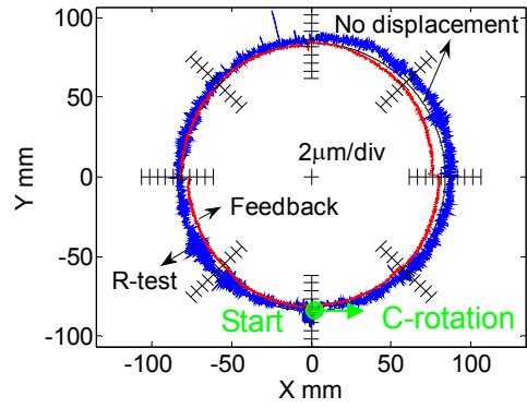
Non-contact R-test
