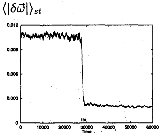
Fig.4, Time evolution of the velocity \langle |\delta \vec{\omega}| \rangle_{st} , calculated at each time step. The time-averaging smooths the line, but does not affect its shape. Initial condition as in Fig.3.
