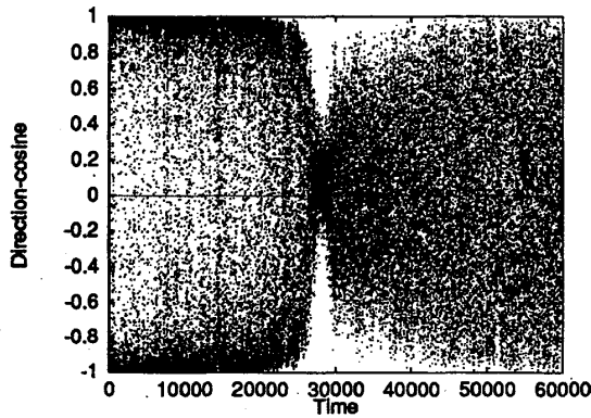
Fig.7, Direction - cosine of \delta\omega for each singular input. Initial condition as in Fig.3.
