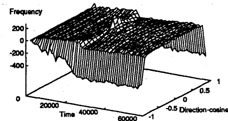
Fig.9, Frequency of Direction - cosines of \delta\omega . The range of Direction - cosine [-1,1] was divided into 20 bins, and counted for each 1000 time steps. (a) Frequency for correlated inputs generated by a tent map. (b) Frequency for random number inputs. (c) Difference of frequencies between (a) and (b). (a) and (b) have the same initial condition as in Fig.3
