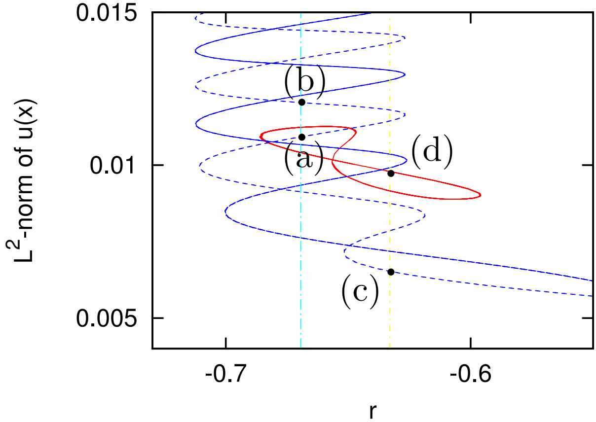
Figure 2.6: (Color online) The snaking branches and isolas projected onto a r - \|u\| plane. The snaking branches consist of two coupled branches, and solutions (a), (b) and (c) belong to the same one of them (dashed blue line). The red (dark gray) figure-eight shaped line denotes the isolas containing the solution (d). Such eight-figured branches can be seen also in two-pulse solutions to SHE [39]. This similarity tells that the solution (d) should be regarded as a connected two-pulse solution.
