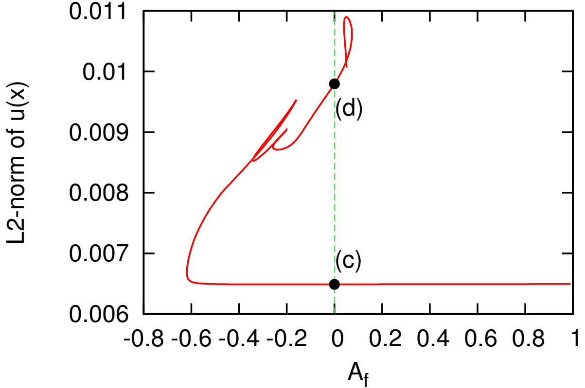
Figure 2.4: (Color online) The trajectory of continuation projected onto A_f - \|u\| started from an unstable solution to the filtered equation. This continuation also cross the line A_f = 0 twice, but a complicated path is realized. Two labeled points (c) and (d) on the line A_f = 0 are also solutions to SHE, and their profiles are shown in Fig. 2.5. As noted in the text a switching between solution branches are occurred in this complicated part of the trajectory.
