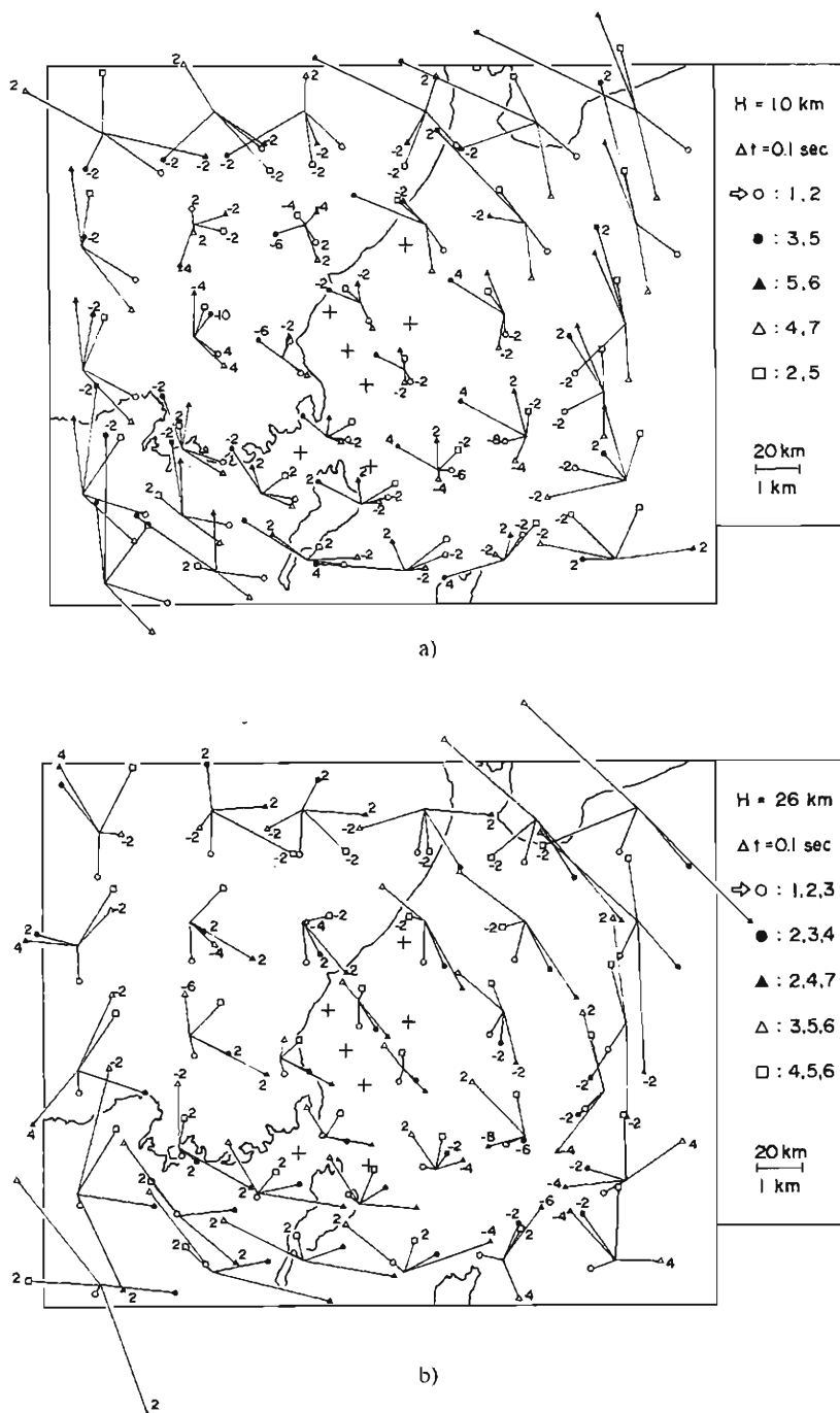
Fig. 9. a) Differences between the fictitious hypocenters and the relocated ones calculated from the data which 0.1 s have been added to each of two P -times. The 5 cases of \gamma C_2 are shown. Each numeral is the same as in Fig. 7. b) Differences between the fictitious hypocenters and the relocated ones calculated from the data which 0.1 s have been added to each of three P -times. The 5 cases of \gamma C_3 are shown. Each numeral is the same as in Fig. 7.
