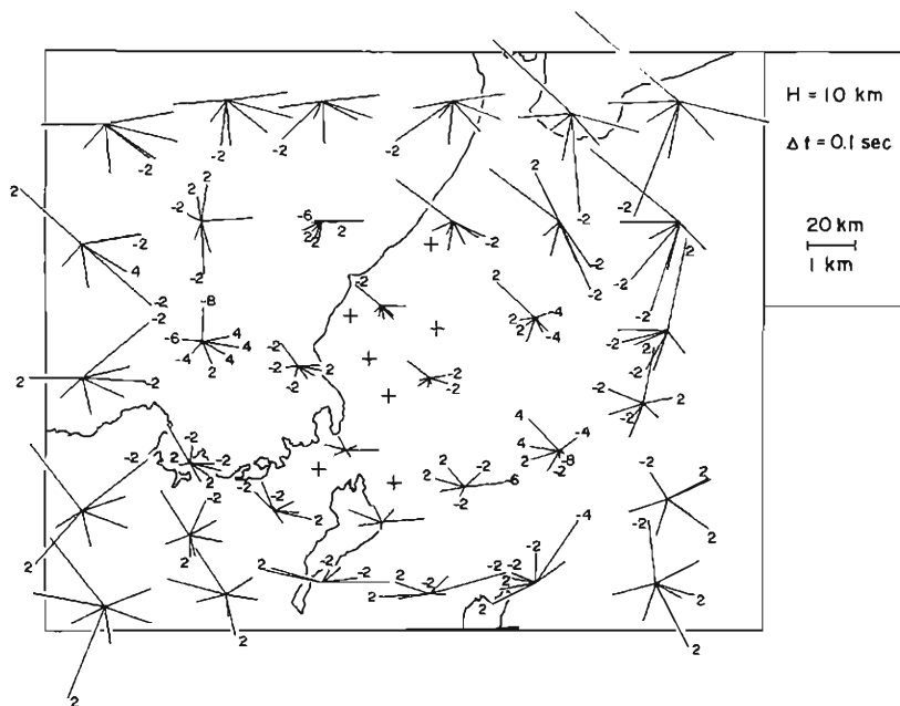
Fig. 7. Differences between the fictitious hypocenters and the relocated ones calculated from the data which 0.1 s is added to one of P -times. The relocated hypocenter depth subtracted by initial one is each numeral at the tip of the line denoted in km.
