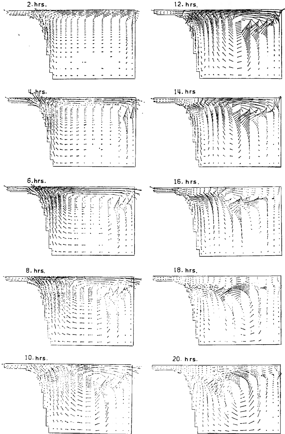
Fig. 6. The velocity distributions illustrated every two hours between t=0 and t=20 hours.
