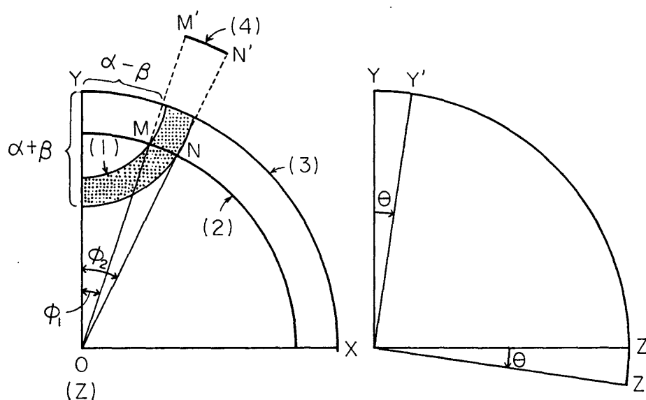
Fig. 1. The interference condition of X-ray and spiral angle. (1) net planeband, (2) refraction circle. (3) Lagenkugel, (4) interference arc, \alpha : spiral angle, \beta : angle between b axis and perpendicular line of lattice plane, OY: axis of symmetry, \theta : BRAGG's angle.
