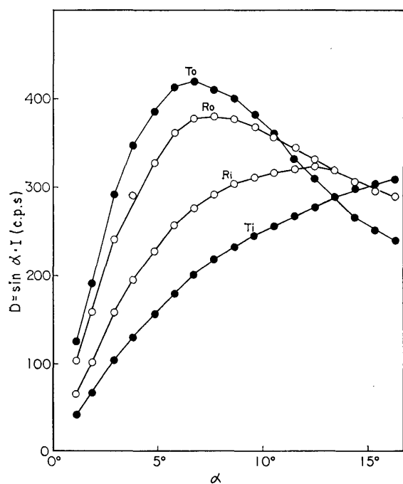
Fig. 2e. Distribution (D) of the angle of micellar orientation of the 50th joint of Mōsō bamboo.
