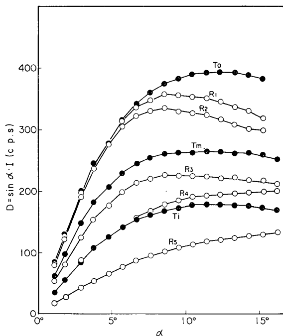
Fig. 2a. Distribution (D) of the angle of micellar orientation of first joint of Mōsō bamboo.
