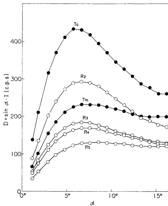
Fig. 2d. Distribution (D) of the angle of micellar orientation of the 30th joint of Mōsō bamboo.
