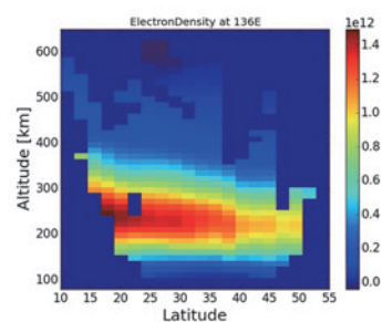
Figure 3. Meridional-height section of the plasma density from 3D tomography at 7:00UT on May 23, 2012.
