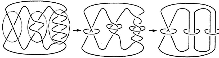
FIGURE 3. (left) a link diagram and its twists. (center) the augmented link diagram. (right) A diagram of a fully augmented link
