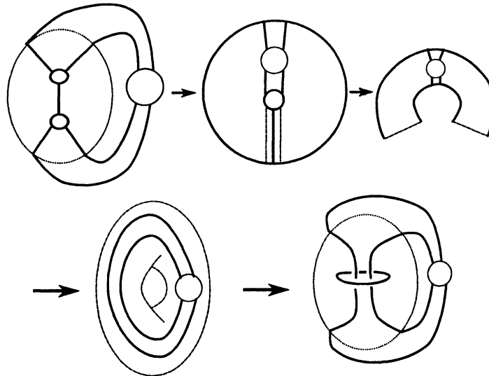
FIGURE 2. Glueing by an automorphism
