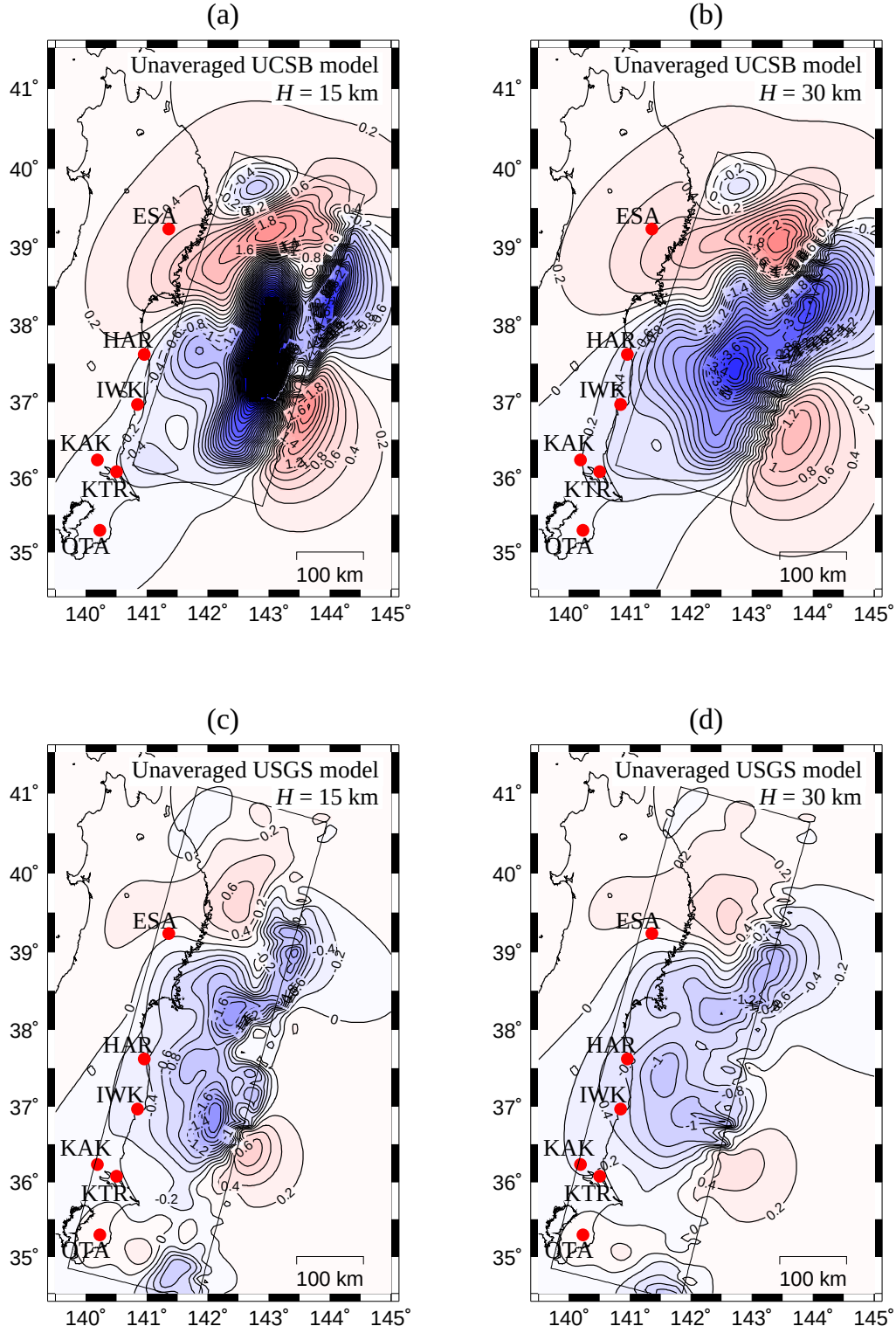
Figure 1 Models of the piezomagnetic field corresponding to the UCSB and USGS slip models. (a) UCSB slip model with H = 15 km. (b) UCSB slip model with H = 30 km. (c) USGS slip model with H = 15 km. (d) USGS slip model with H = 30 km. The rectangle represents the fault plane on which heterogeneous slip is considered.
