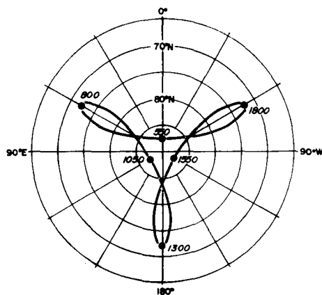
Fig. 20. The model of a hypothetical wobbling motion of the geomagnetic dipole axis. (After KAWAI and HIROOKA, 1967)
