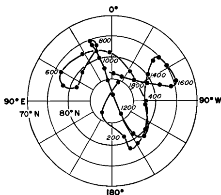
Fig. 16. Virtual pole positions calculated from each set of the mean inclination and the mean declination for every 50 years.
