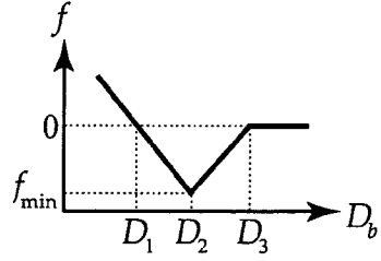
Fig. 9 Attractive or repulsive force working between cylinders (the horizontal axis shows the distance between the centers of two cylinders)
