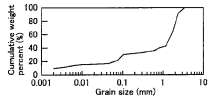
Fig. 4 Grain size distribution in the experimental material
