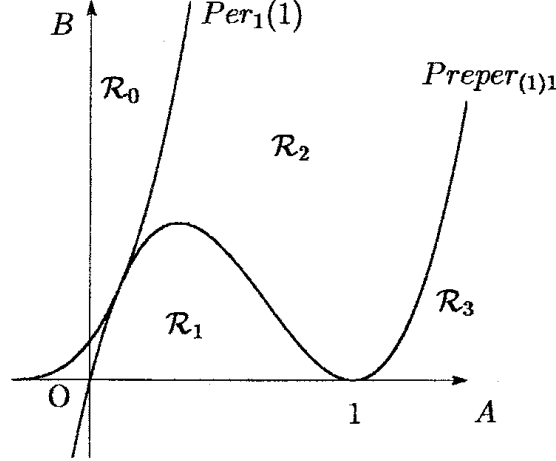
Figure 1: Parameter space for real cubics
