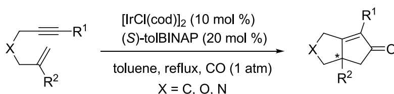
Scheme 9. Iridium-catalyzed enantioselective Pauson-Khand-type reaction of enynes.
