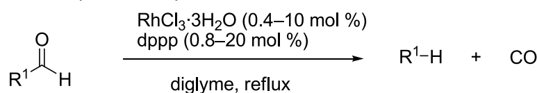
Scheme 1-2. Rhodium-mediated or -catalyzed decarbonylation of aldehydes.
