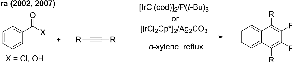
Scheme 5-2. Transition-metal-mediated annulative condensation on a phenyl ring.
