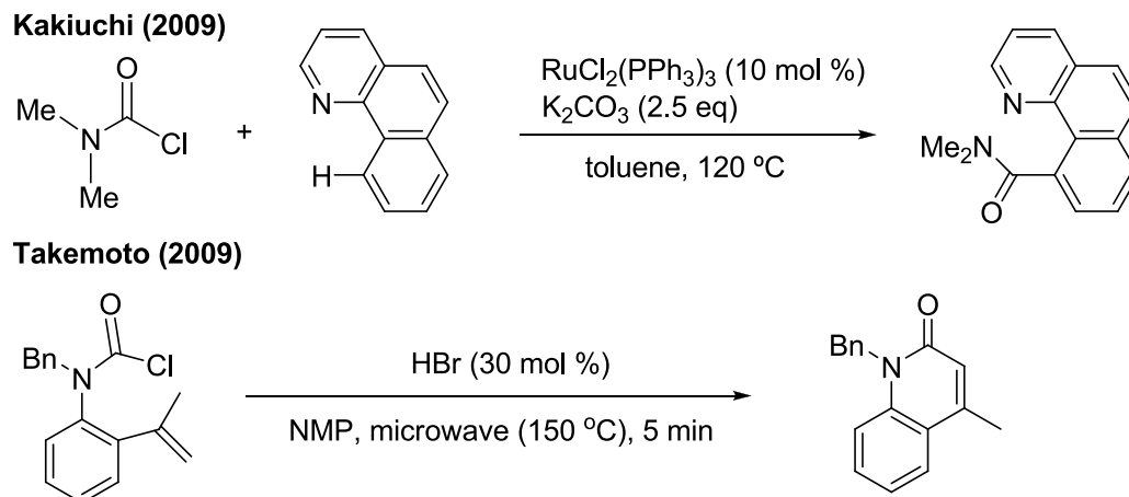
Scheme 4-2. Synthetic methods using carbamoyl chlorides as the substrates.
