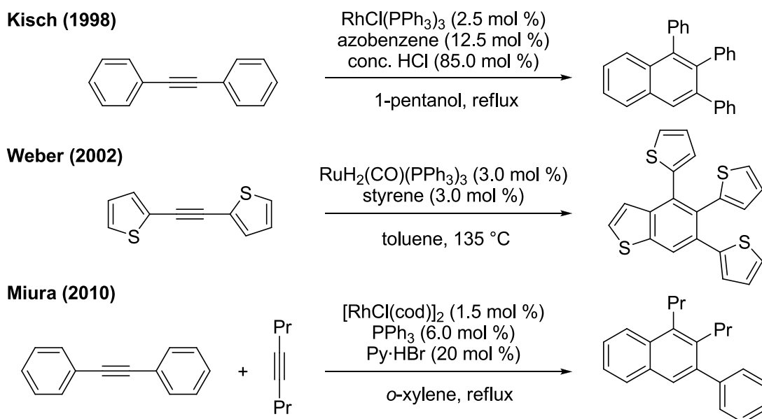
Scheme 5-3. Transition-metal-catalyzed cyclodimerization of alkynes.
