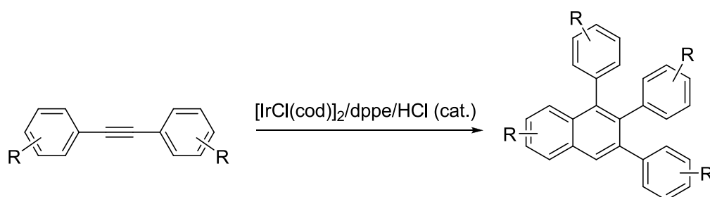
Scheme 17. Iridium-catalyzed cyclodimerization of diarylacetylenes.
