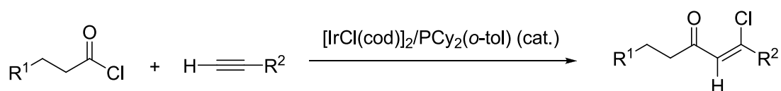
Scheme 15. Iridium-catalyzed addition of aliphatic acid chlorides to terminal alkynes.
