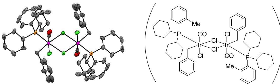
Figure 3-1. Single crystal structure of 4 .
