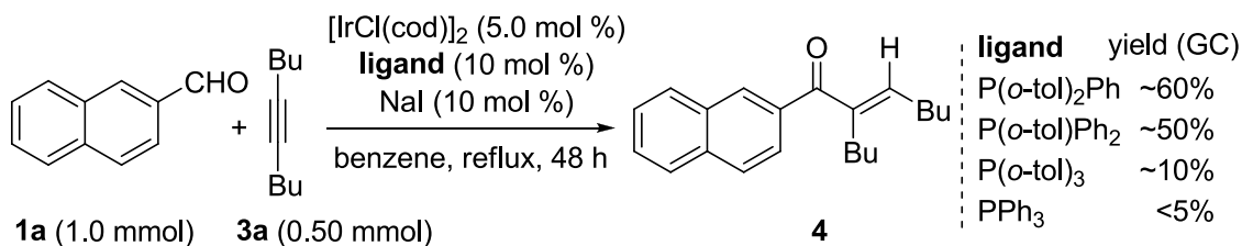
Scheme 1-3. Iridium-catalyzed hydroacylation of 5-decyne with 2-naphthaldehyde.
