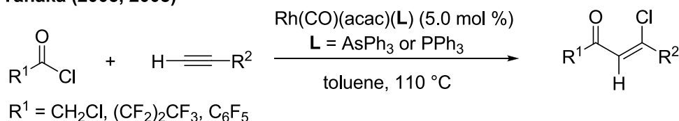
Scheme 2-2. Rhodium-catalyzed addition of acid chlorides to terminal alkynes.
