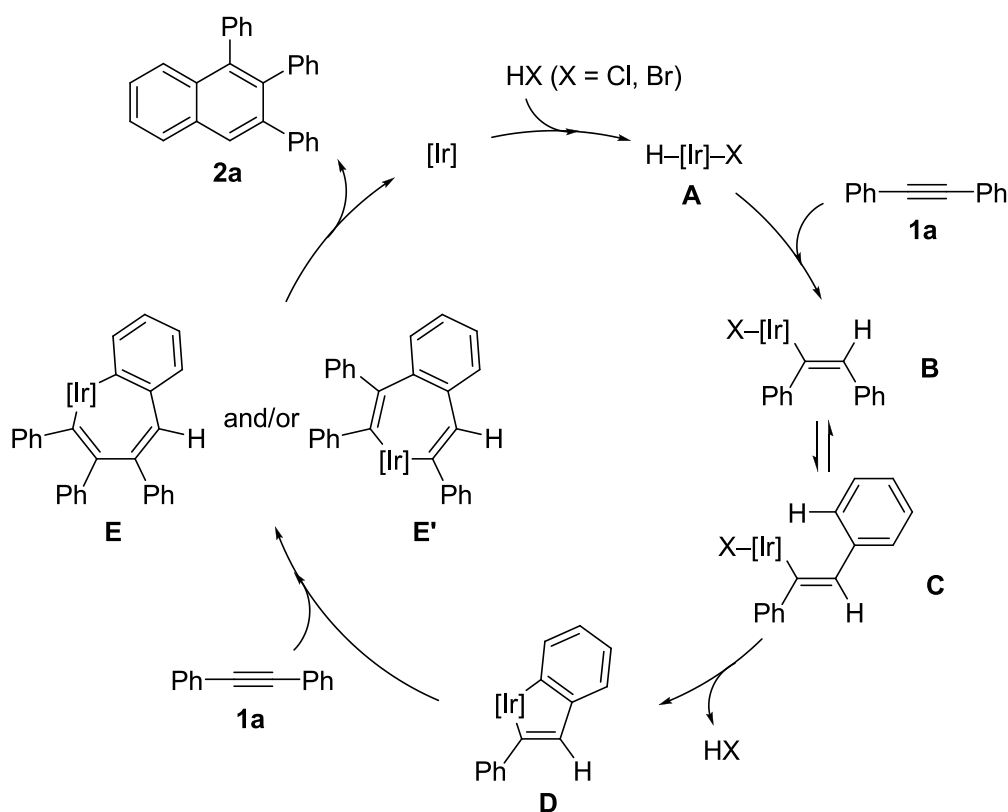
Scheme 5-7. Plausible reaction mechanism.
