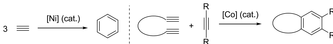
Scheme 5-1. [2+2+2] Cyclotrimerization of alkynes.
