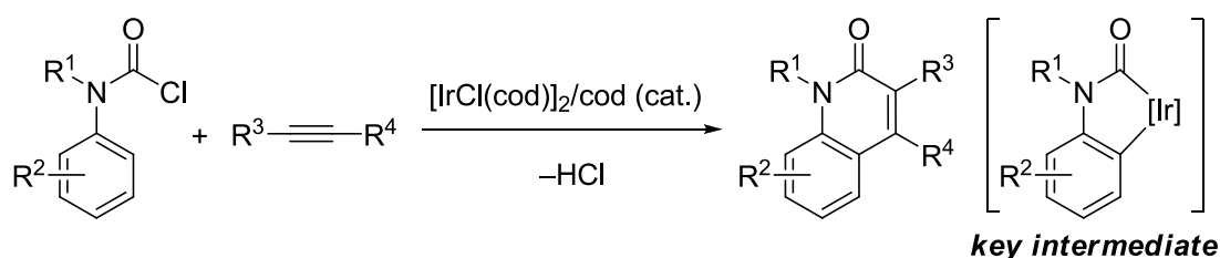
Scheme 16. Iridium-catalyzed annulation of N -arylcabamoyl chlorides with internal alkynes.
