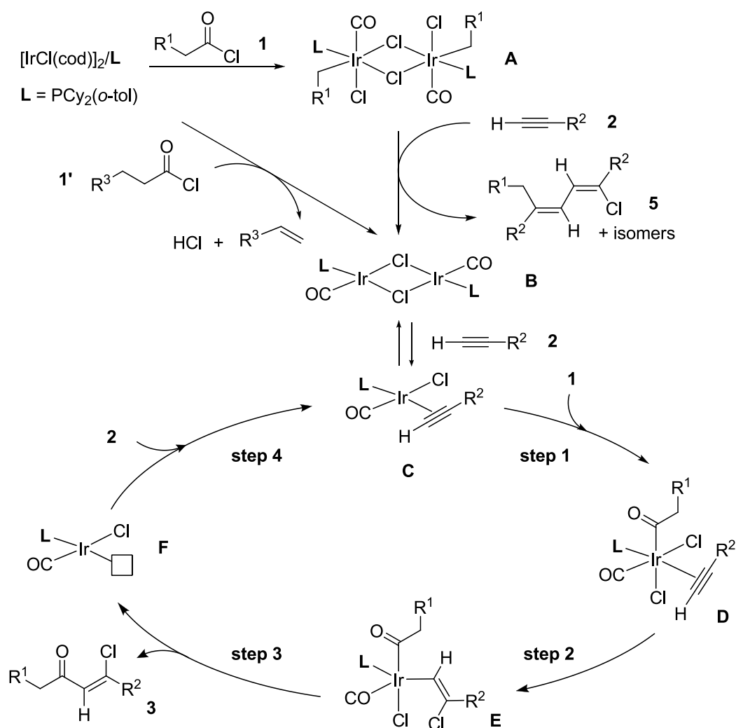
Scheme 3-1. Plausible reaction mechanism.
