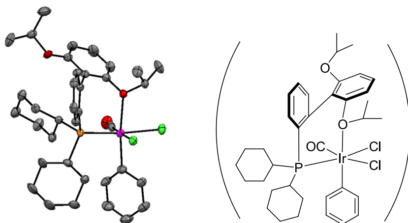
Figure 2-1. Crystal structure of 6 .
