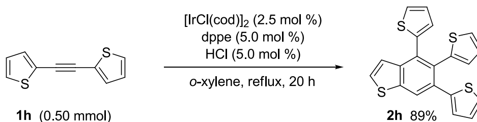
Scheme 5-5. Iridium-catalyzed cyclodimerization of 1h .
