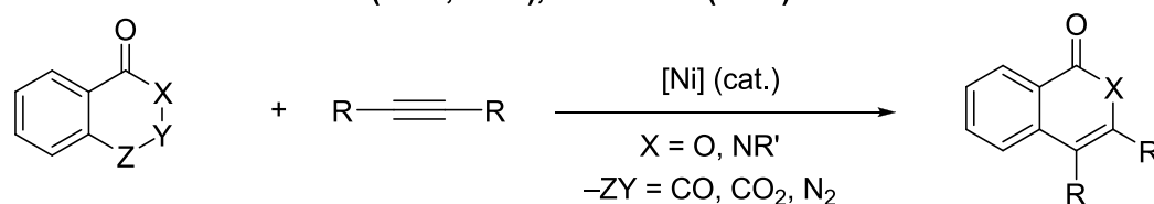
Scheme 4-1. Several synthetic methods for carbonyl-containing N -heterocycles.
