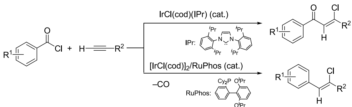
Scheme 13. Iridium-catalyzed addition of aromatic acid chlorides to terminal alkynes.
