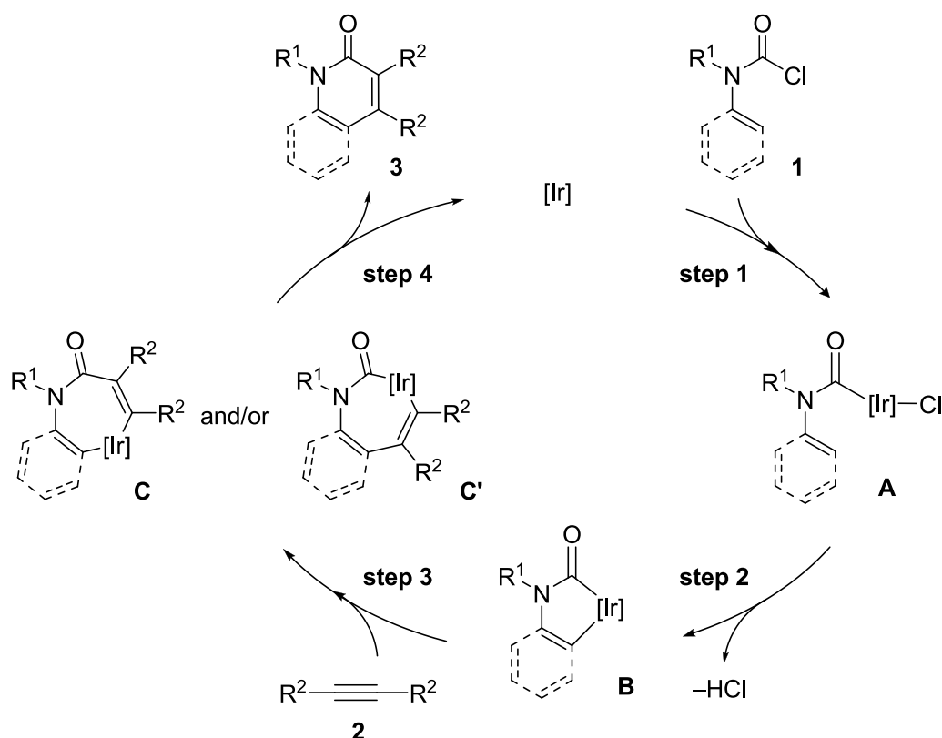
Scheme 4-4. Plausible reaction mechanism.
