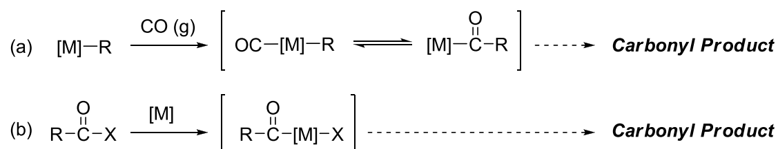
Scheme 1. General reaction types of transition-metal-catalyzed transformation of carbonyl functionalities.
