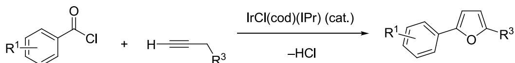
Scheme 14. Iridium-catalyzed synthesis of 2,5-disubstituted furans.
