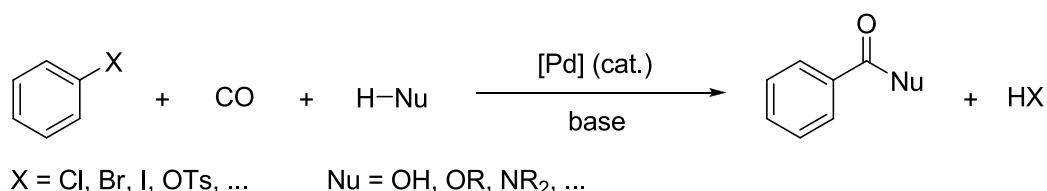
Scheme 2. Palladium-catalyzed carbonylation of aryl halides with various nucleophiles.
