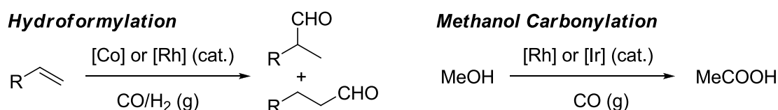
Scheme 4. Hydroformylation and methanol carbonylation.
