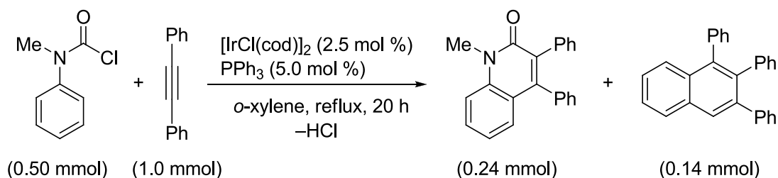
Scheme 5-4. The reaction of N -methyl- N -phenylcarbamoyl chloride and diphenylacetylene in the presence of the iridium catalyst.
