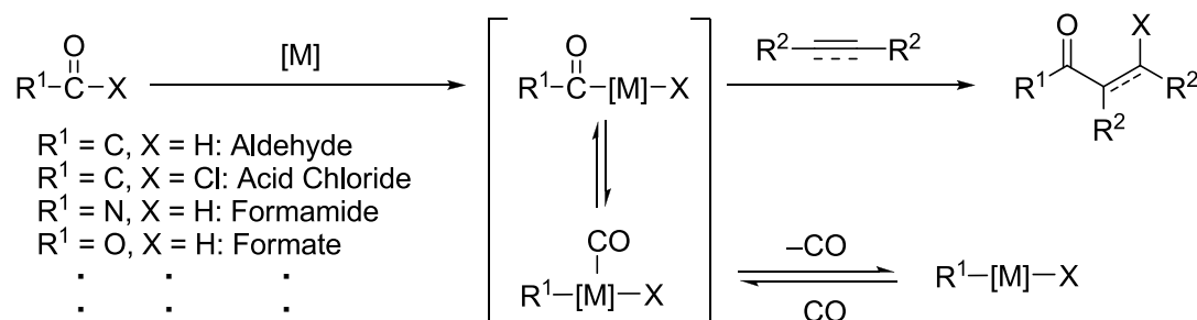
Scheme 5. Additions of carbonyl functionalities to carbon-carbon multiple bonds.
