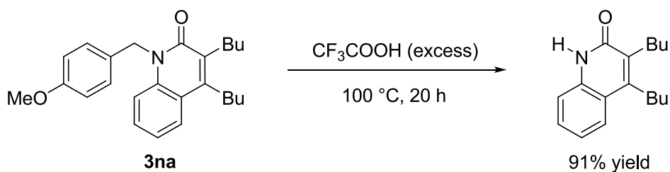
Scheme 4-3. Deprotection of the 4-methoxyphenylmethyl group on 3na .
