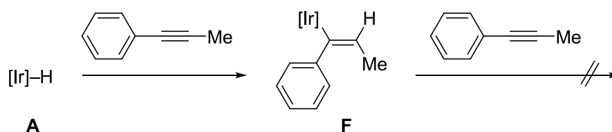
Scheme 5-8. Insertion of aryl-alkylacetylenes to the iridium-hydride species A .
