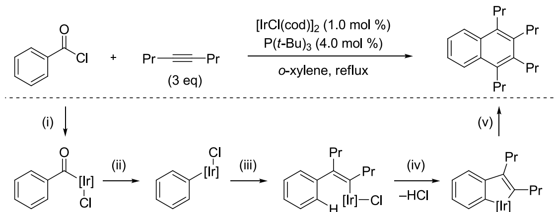
Scheme 11. Iridium-catalyzed reaction of aroyl chlorides with internal alkynes.
