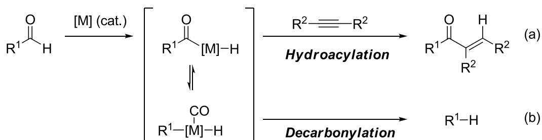
Scheme 1-1. Transition-metal-catalyzed reactions of aldehydes.
