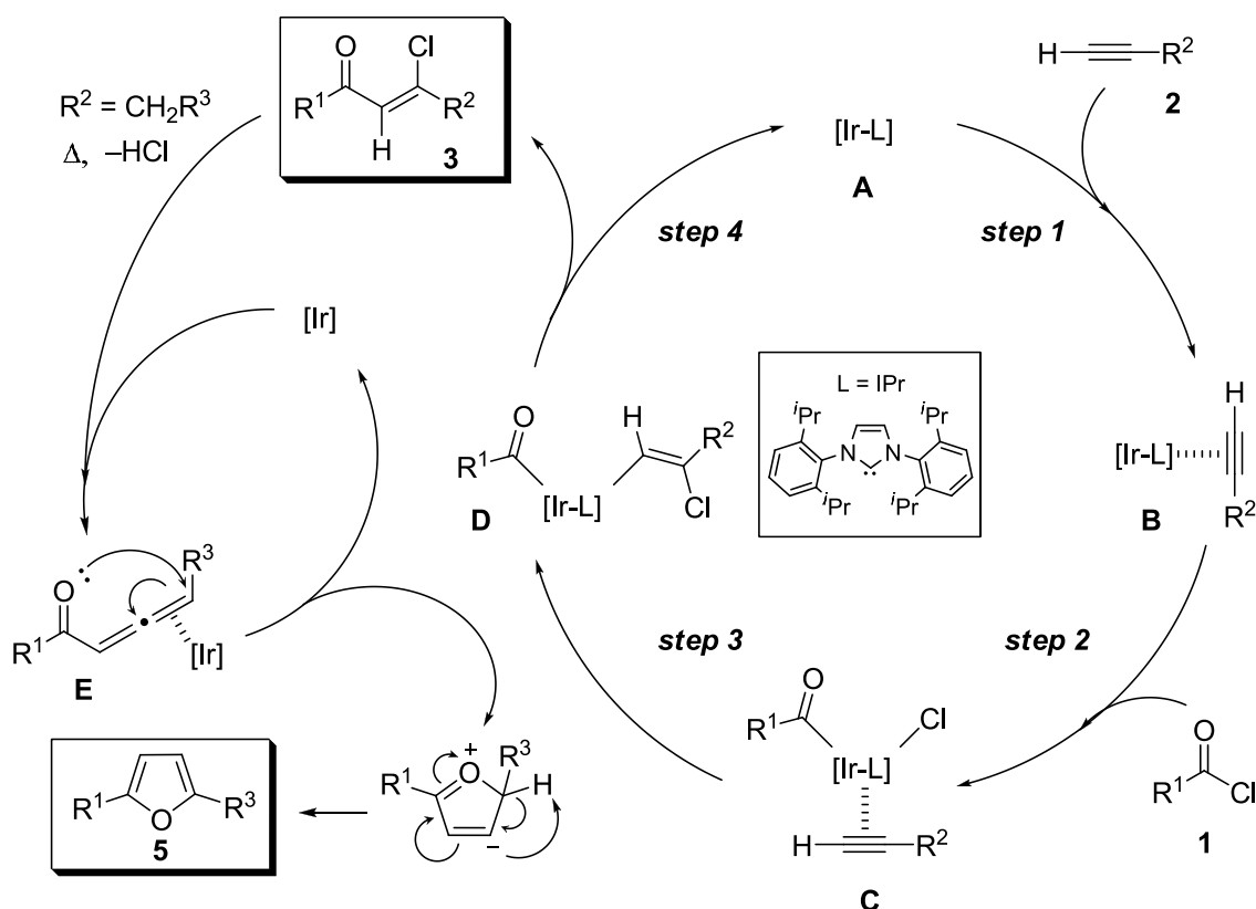
Scheme 2-3. A plausible catalytic cycle for the iridium-catalyzed addition of acid chlorides to terminal alkynes.
