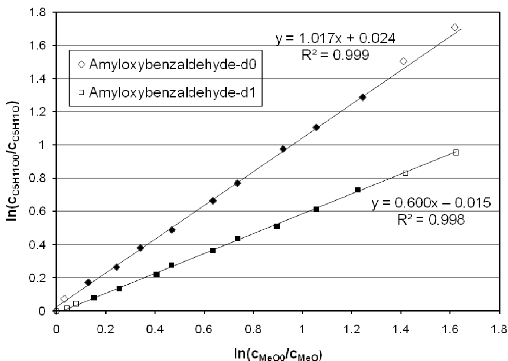
Figure 1-1. The kinetic isotope effect ( k_H/k_D ) measurement for the 4-amyloxybenzaldehydes.
