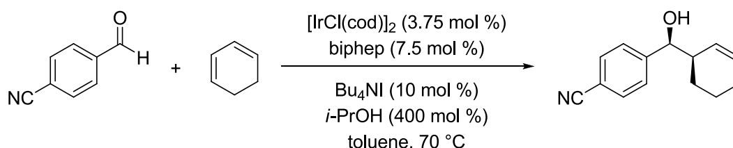
Scheme 10. Iridium-catalyzed transfer hydrogenative coupling of 1,3-diene and aldehyde.
