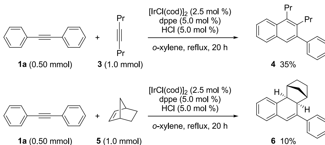
Scheme 5-6. Iridium-catalyzed cross-dimerization of 1a with 4-octyne or norbornene.
