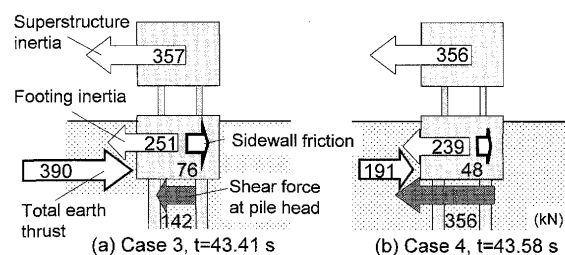
Fig. 11. Forces acting on piles-footing-superstructure system
