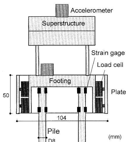
Fig. 3. Piles-footing-superstructure model
