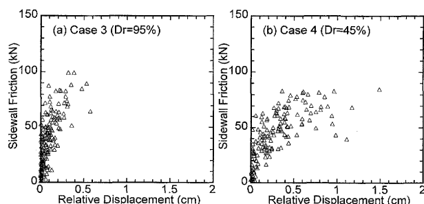
Fig. 16. Relation between relative displacement and sidewall friction peak
