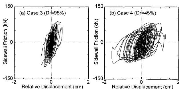
Fig. 15. Relation between relative displacement and sidewall friction
