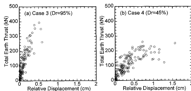
Fig. 14. Relation between relative displacement and total earth thrust peak
