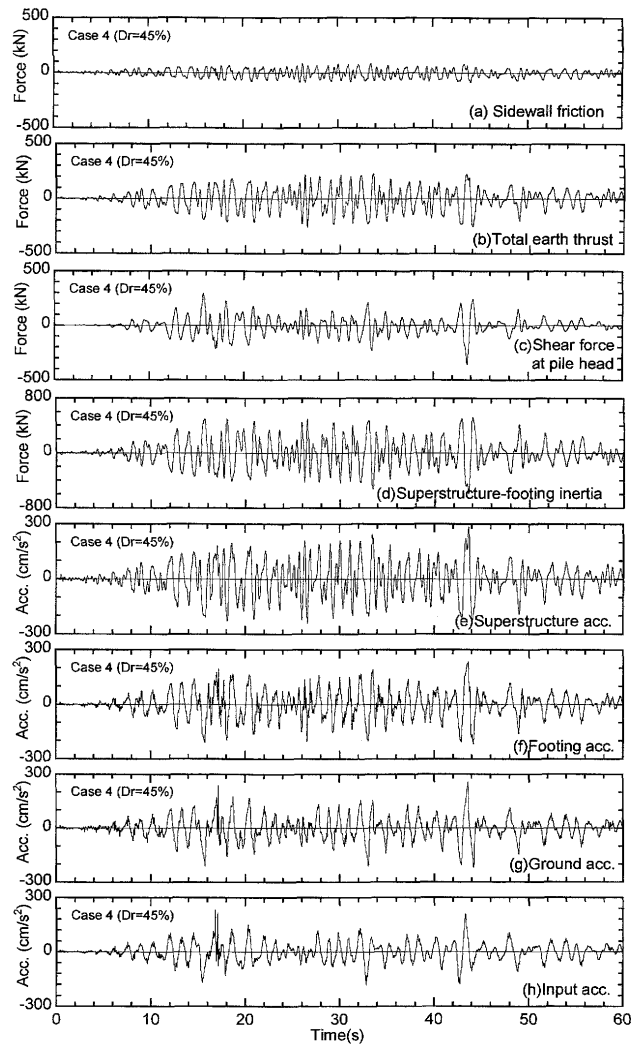
Fig. 7. Time histories in Case 4 (Loose sand)
