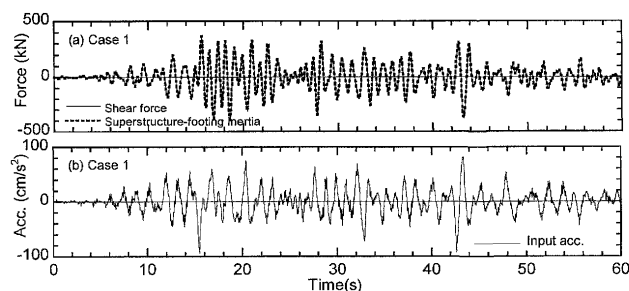
Fig. 4. Time histories in Case 1
