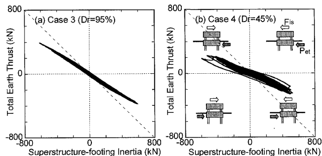
Fig. 9. Relation between superstructure-footing inertia and total earth thrust
