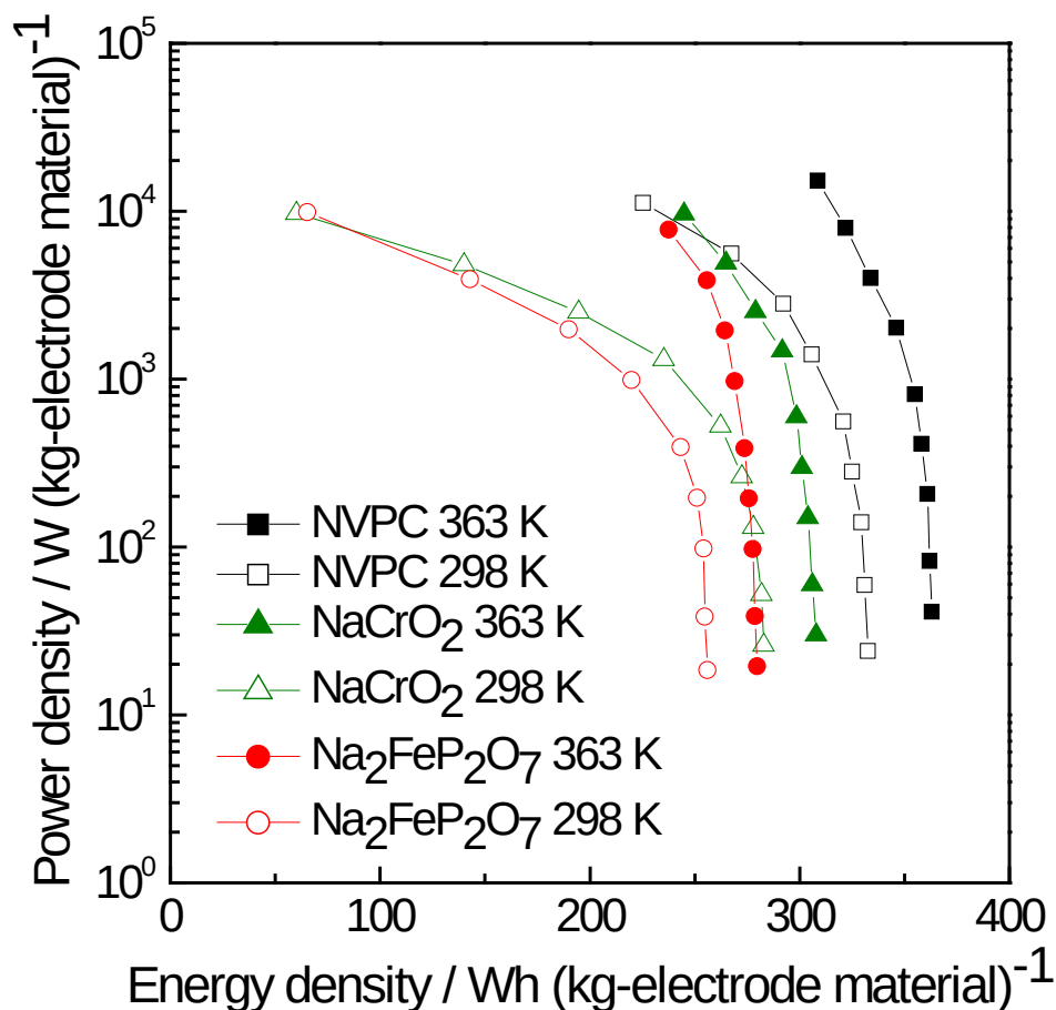
Figure 11 Relationships between power and energy densities for NVPC, \text{Na}_2\text{FeP}_2\text{O}_7 , and \text{NaCrO}_2 with \text{Na}[\text{FSA}]\text{--}[\text{C}_2\text{C}_{11}\text{im}][\text{FSA}] IL electrolytes based on rate capability tests ( \text{Na}[\text{FSA}] mole fraction = 0.3 at 298 K and \text{Na}[\text{FSA}] mole fraction = 0.5 at 363 K). Power and energy densities are calculated based on the weight of the positive electrode, assuming Na metal negative electrode.
