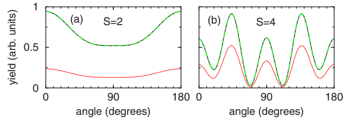
FIG. 8. (Color online) Photoelectron angular distributions at the different photoelectron energies by the chirped pulses with the chirp rates of \xi = -\sqrt{15} (solid), \xi = 0 (thin solid), and \xi = \sqrt{15} (dot-dashed). The orders of the ATI peaks are (a) S=2 and (b) S=4 as labeled in Fig. 7. The photon energy is 6.2 eV and \tau_{\text{TL}} = 6.65 fs for the transform-limited pulse. After the appropriate normalization all the PADs in each panel become practically identical.
