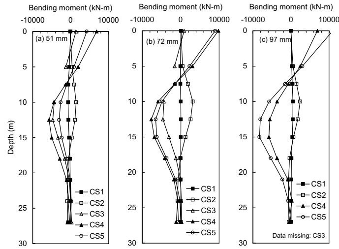
Fig. 6 Vertical profile of bending moment when the pile head displacement is absolute maximum.
