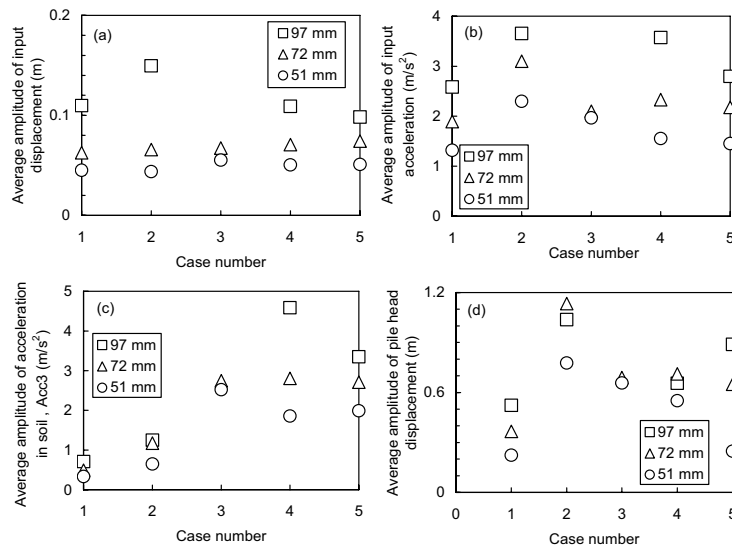
Fig. 5 Average amplitude of input displacement (a), input acceleration (b), acceleration in soil, Acc3 (c), and pile head displacement (d).
