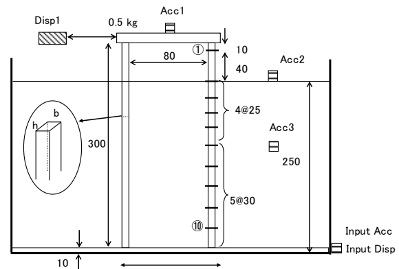
Fig. 2 Cross section of centrifuge model (Units are in mm: model scale)
