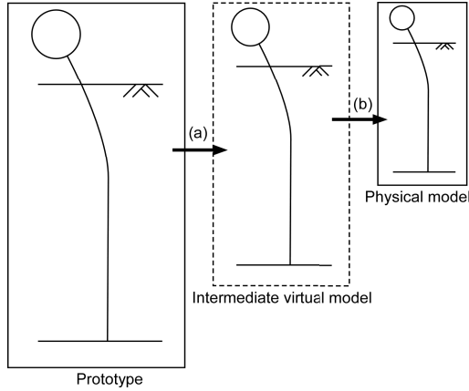
Fig. 1 Concept of two stage scaling: (a) scaling relations for 1g field; (b) scaling relations for centrifugal field (modified after Iai et al., 2005).
