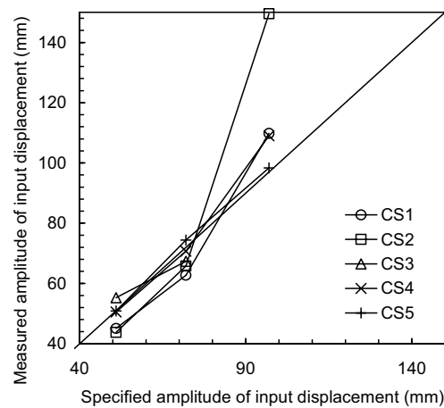
Fig. 4 Specified versus measured amplitude of input displacement. Amplitude is an average.
