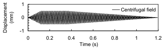
Fig. 3 Example of input displacement in centrifugal field.
