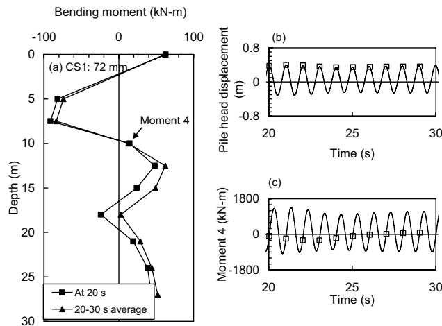
Fig. 7 Vertical profile of bending moment of CS1 (specified input displacement amplitude of 72 mm) (a) , time histories of pile head displacement (b) and bending moment of Moment 4 (c).
