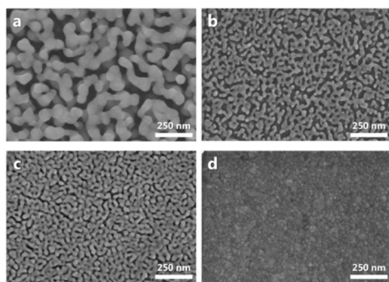
Fig. 1. SEM images of nanoporous gold (NPG-a, NPG-b and NPG-c) (a–c) and flat gold (FG) (d).
