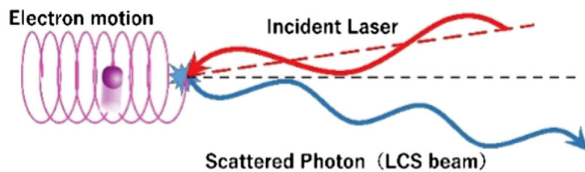
FIG. 1. Conceptual drawing of F-LCS beam generation.
