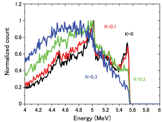
FIG. 6. LCS energy spectra calculated EGS5 including Ge detector response.
