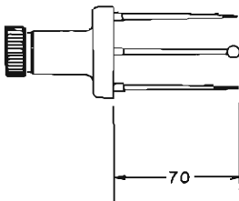
Fig. 9. Sensor of the pulse-time difference flowmeter (mm).
