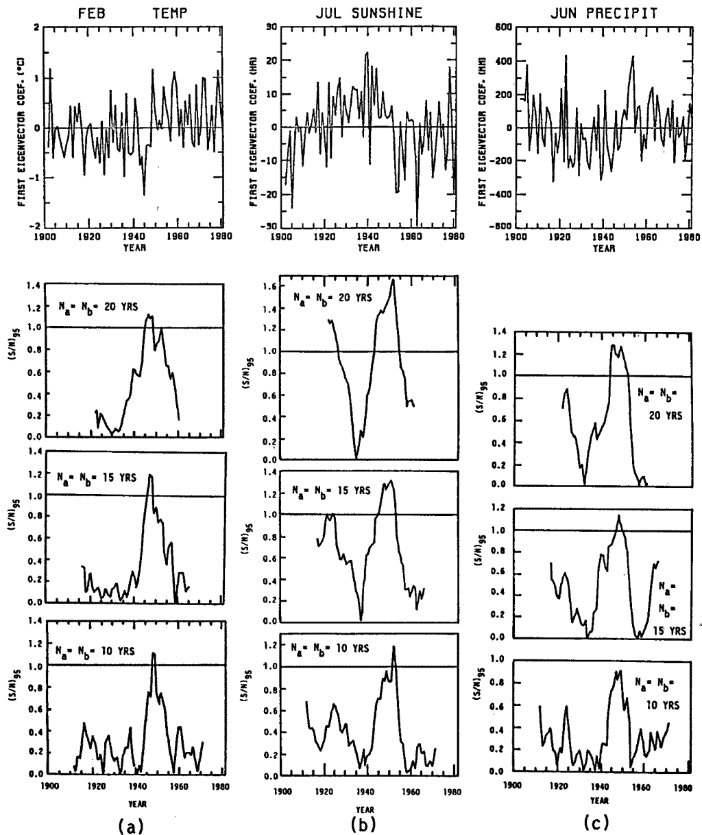
Fig. 1. Detection of climatic jump for the coefficient of the first eigenvector: (a) surface air temperature over Japan in February; (b) sunshine duration over Japan in July; and (c) precipitation over Japan in June. The time coefficient is shown in the top panel. Signal/noise ratios for 95% confidence limit for averaging intervals of 20, 15 and 10 years are shown in the lower 3 panels, respectively.
